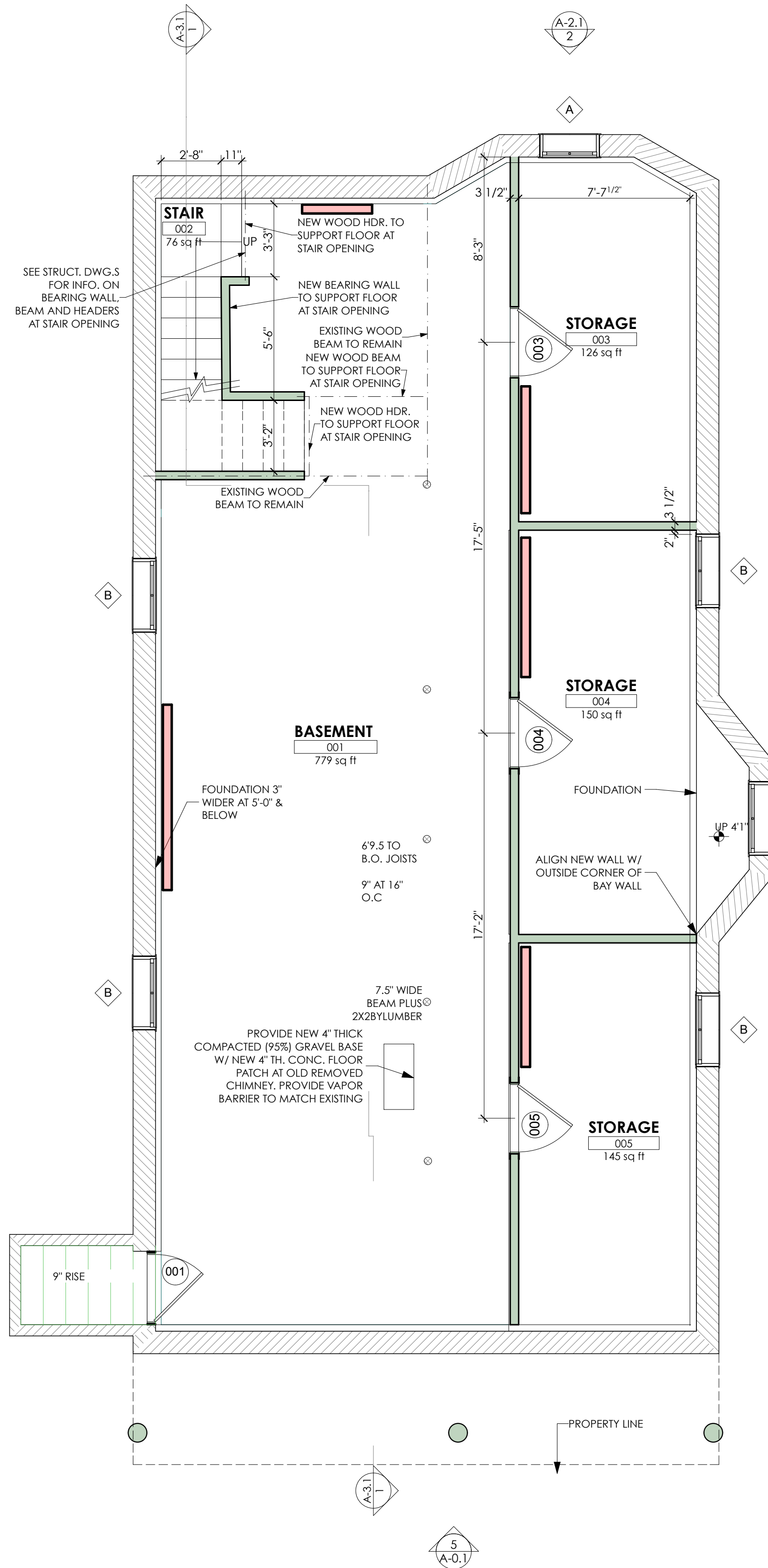
1 BASEMENT SCALE: 1/4" = 1'-0"
