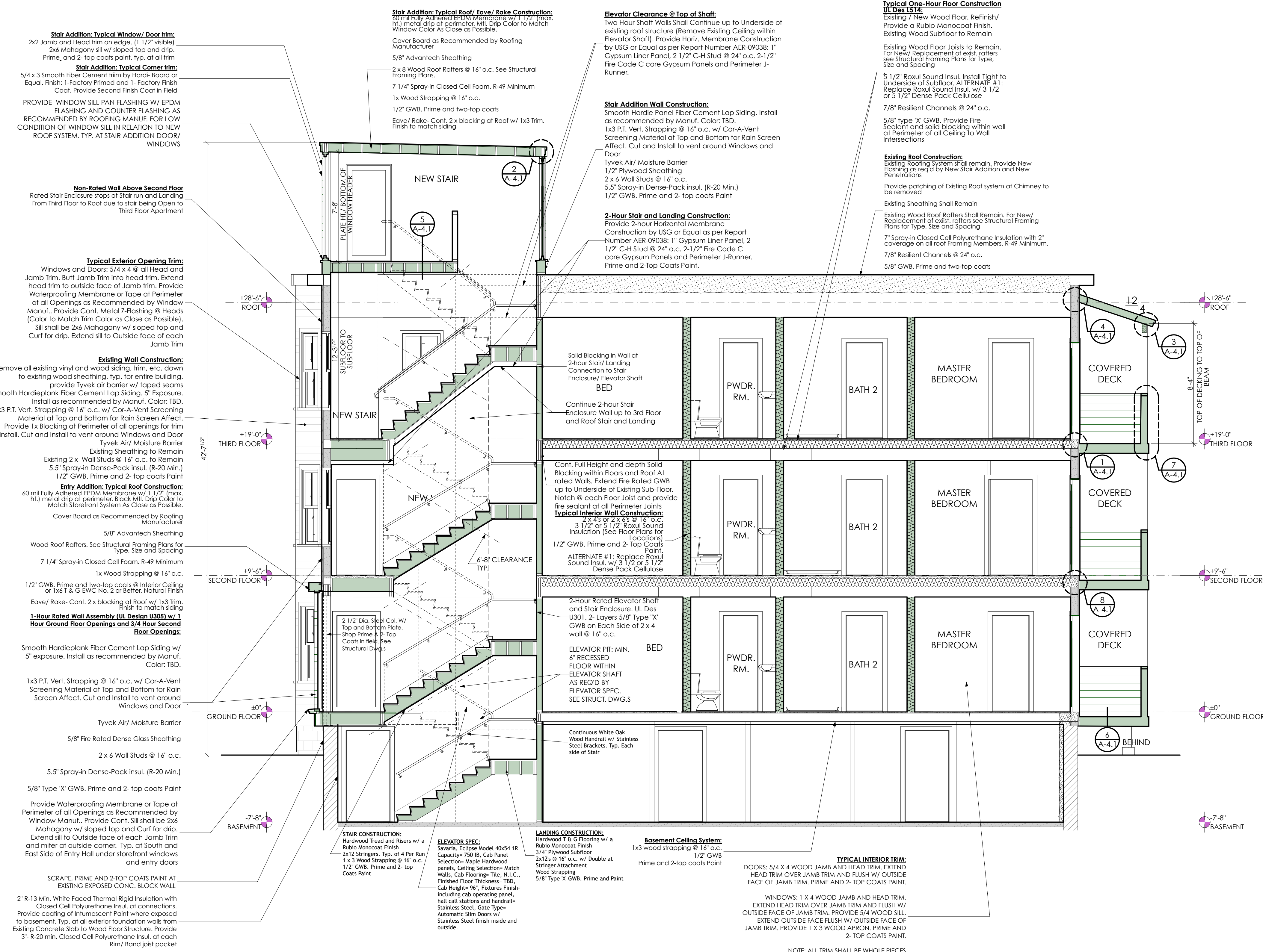
1 PROPOSED LONGITUDINAL SECTION SCALE: 1/4" = 1'-0" 0 2 4 8
