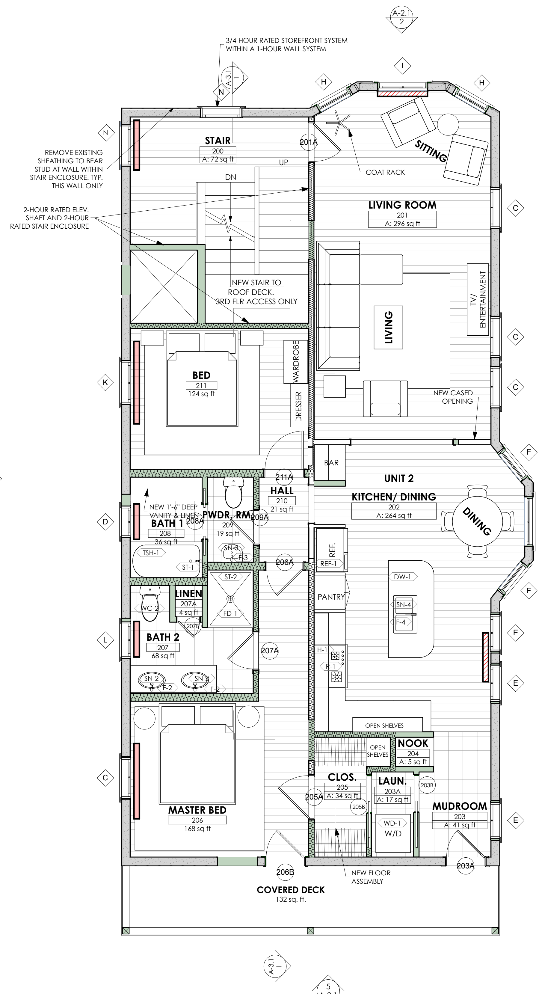
3 SECOND FLOOR SCALE: 1/4" = 1'-0"
