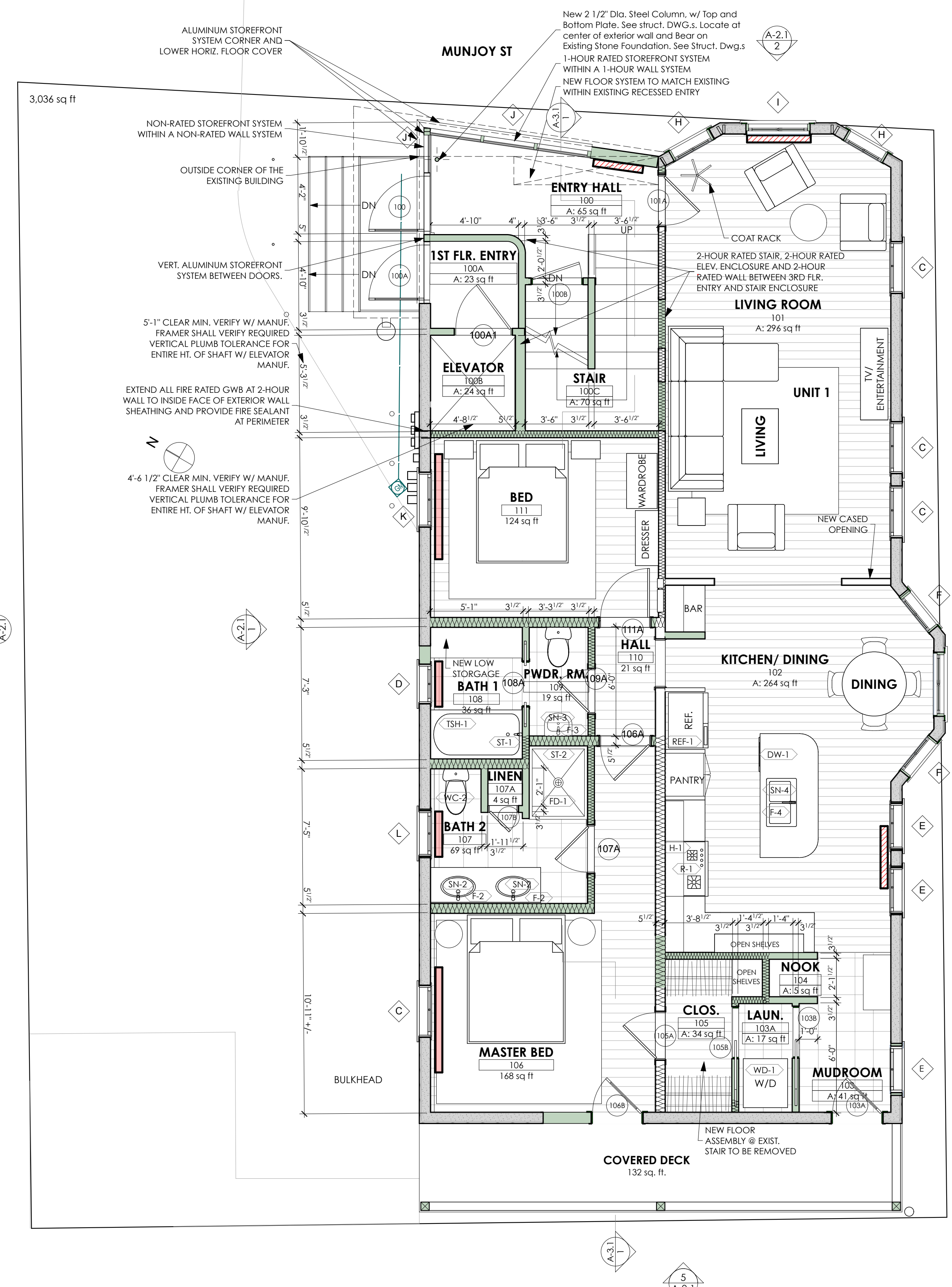
2 GROUND FLOOR SCALE: 1/4" = 1'-0"
