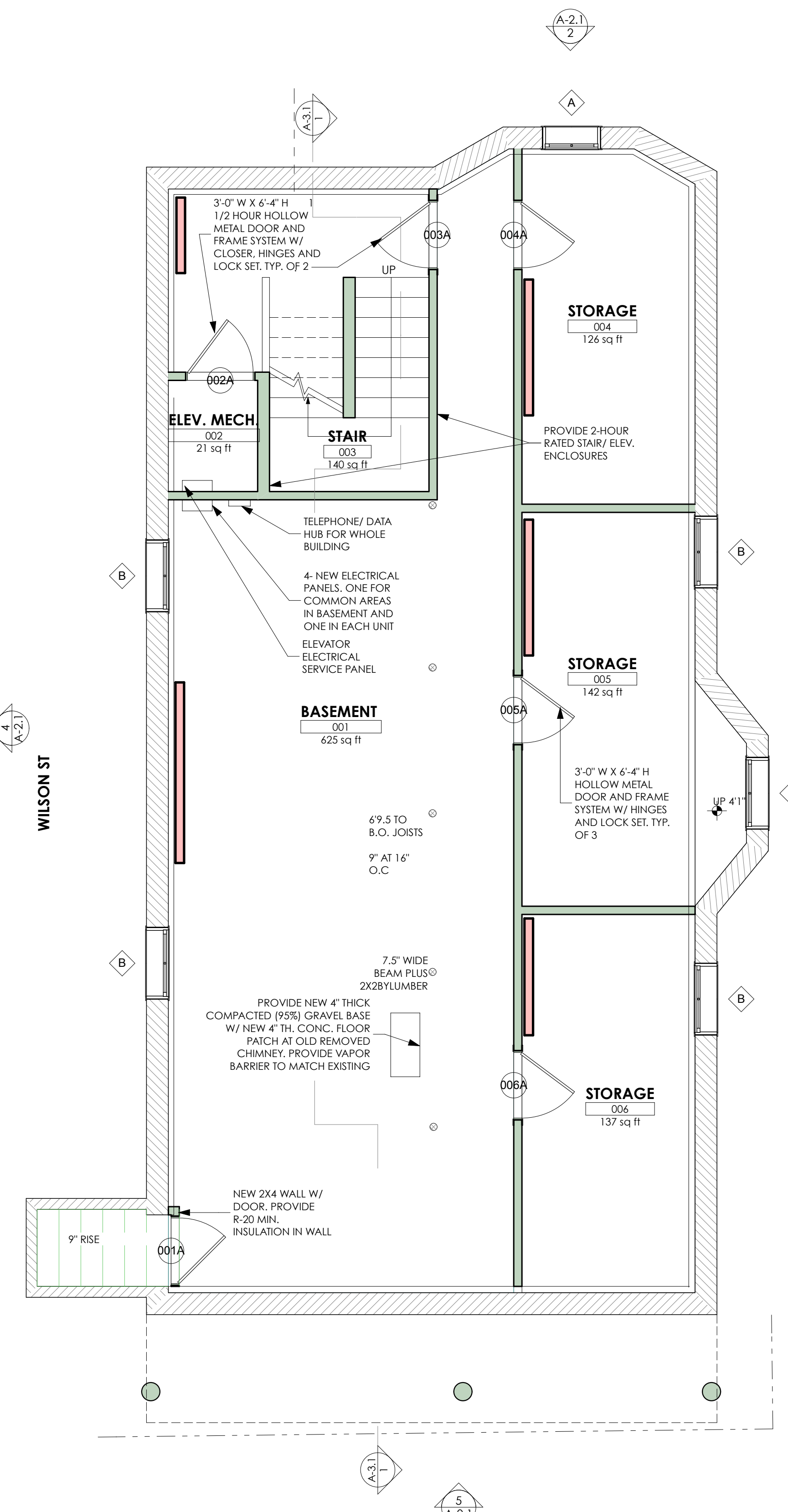
1 BASEMENT SCALE: 1/4" = 1'-0"
