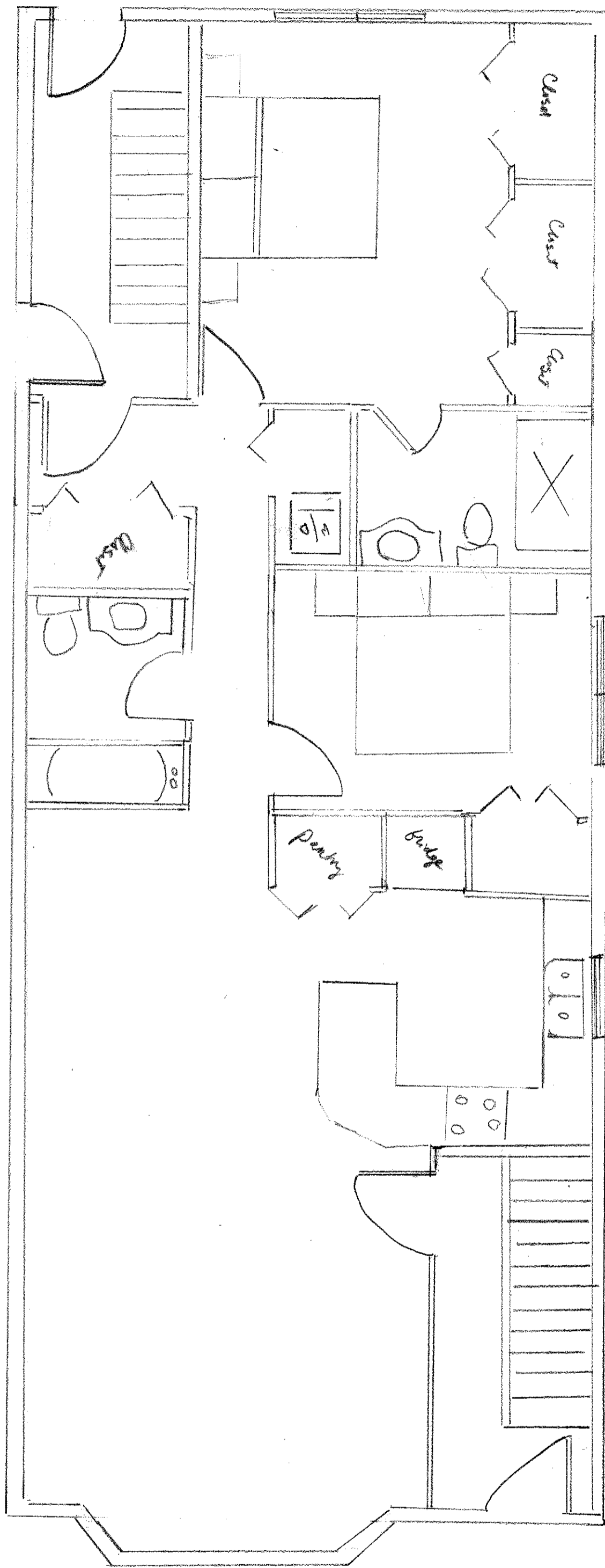
Proposed Floor Plan
