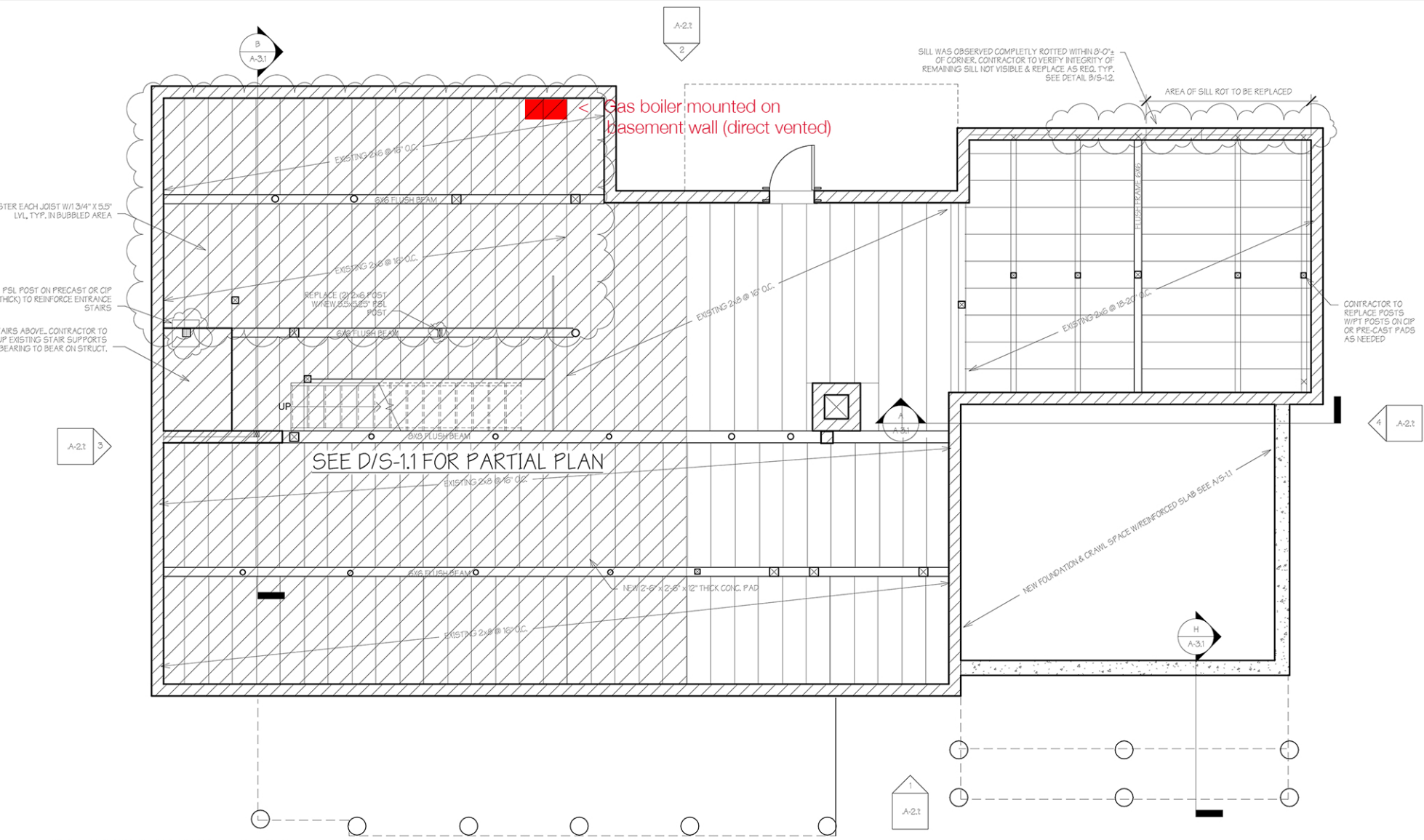
EXISTING BASEMENT & FRAMING + REINFORCEMENT PLAN 1/4" = 1'-0"
