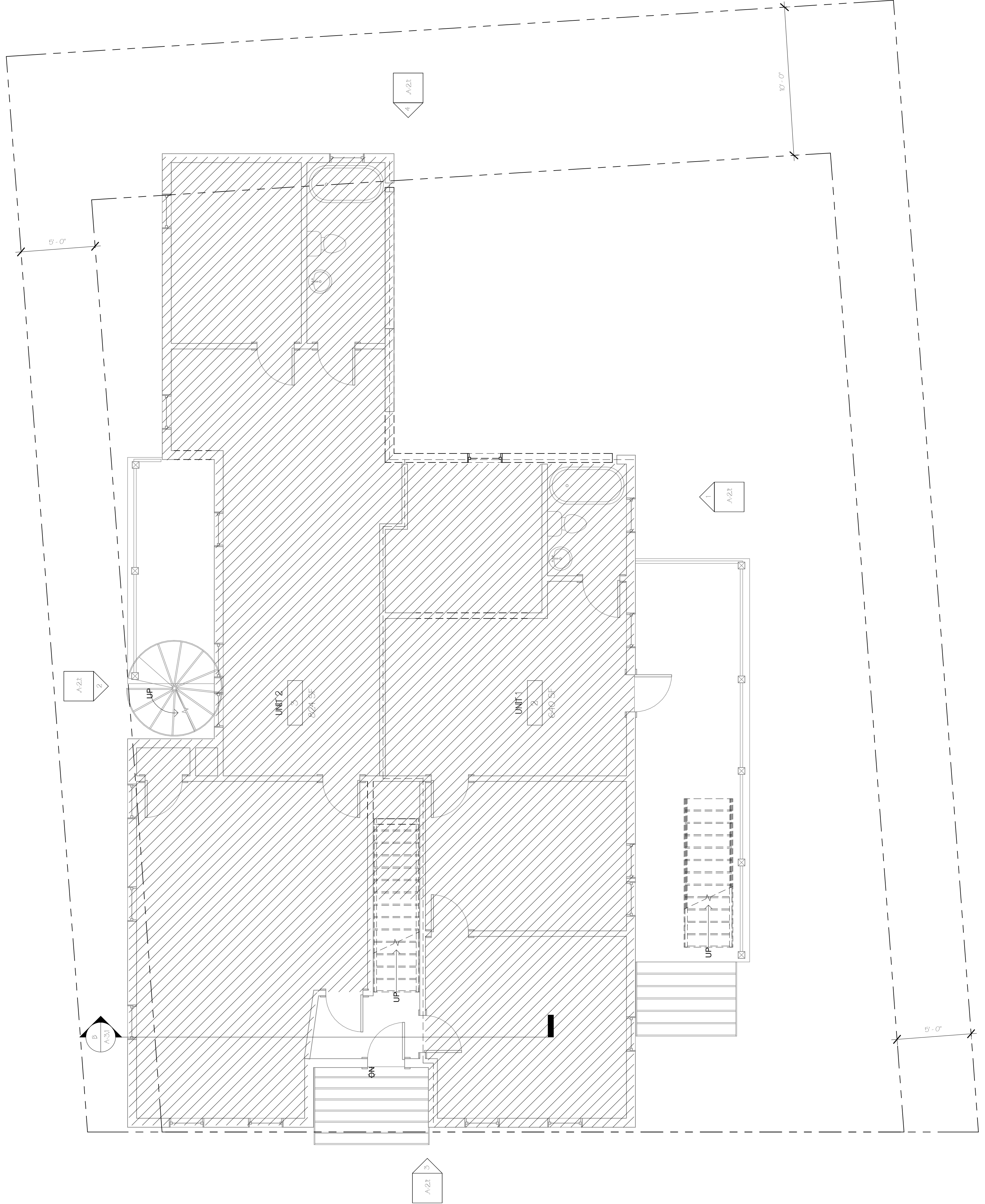
2 First Floor Existing/Demo 1/4" = 1'-0"
