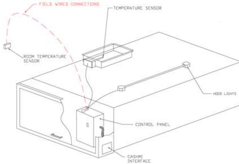
TYPICAL SC CONTROL SYSTEM WITH HOOD MOUNTED PANEL
