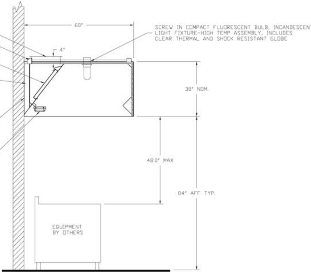
SECTION VIEW - MODEL 6030ND-2 HOOD - #1
