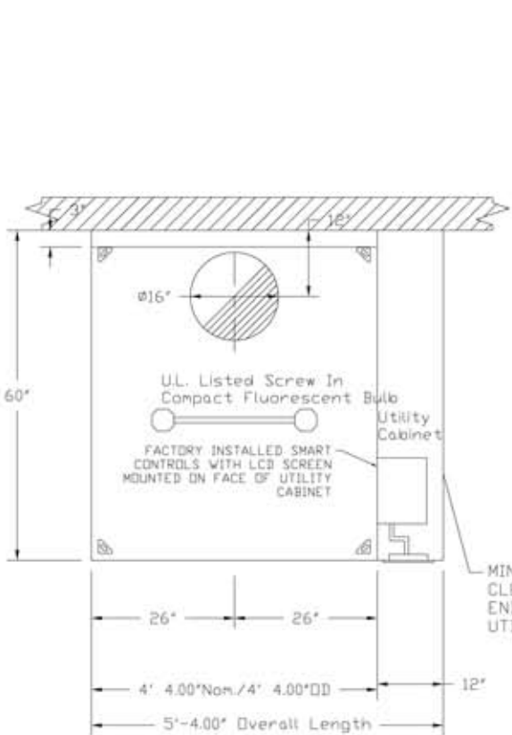
PLAN VIEW - Hood #1 4' 4.00" LONG 6030ND-2
