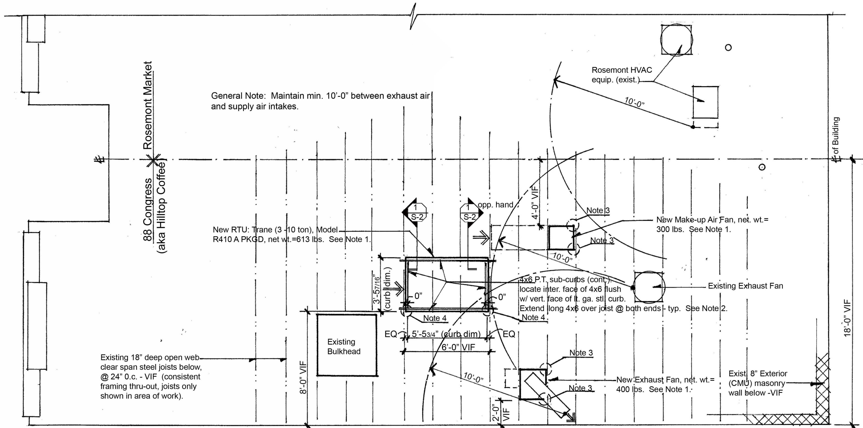
1 Roof & Rooftop Equipment Plan 1/4" = 1'-0"
