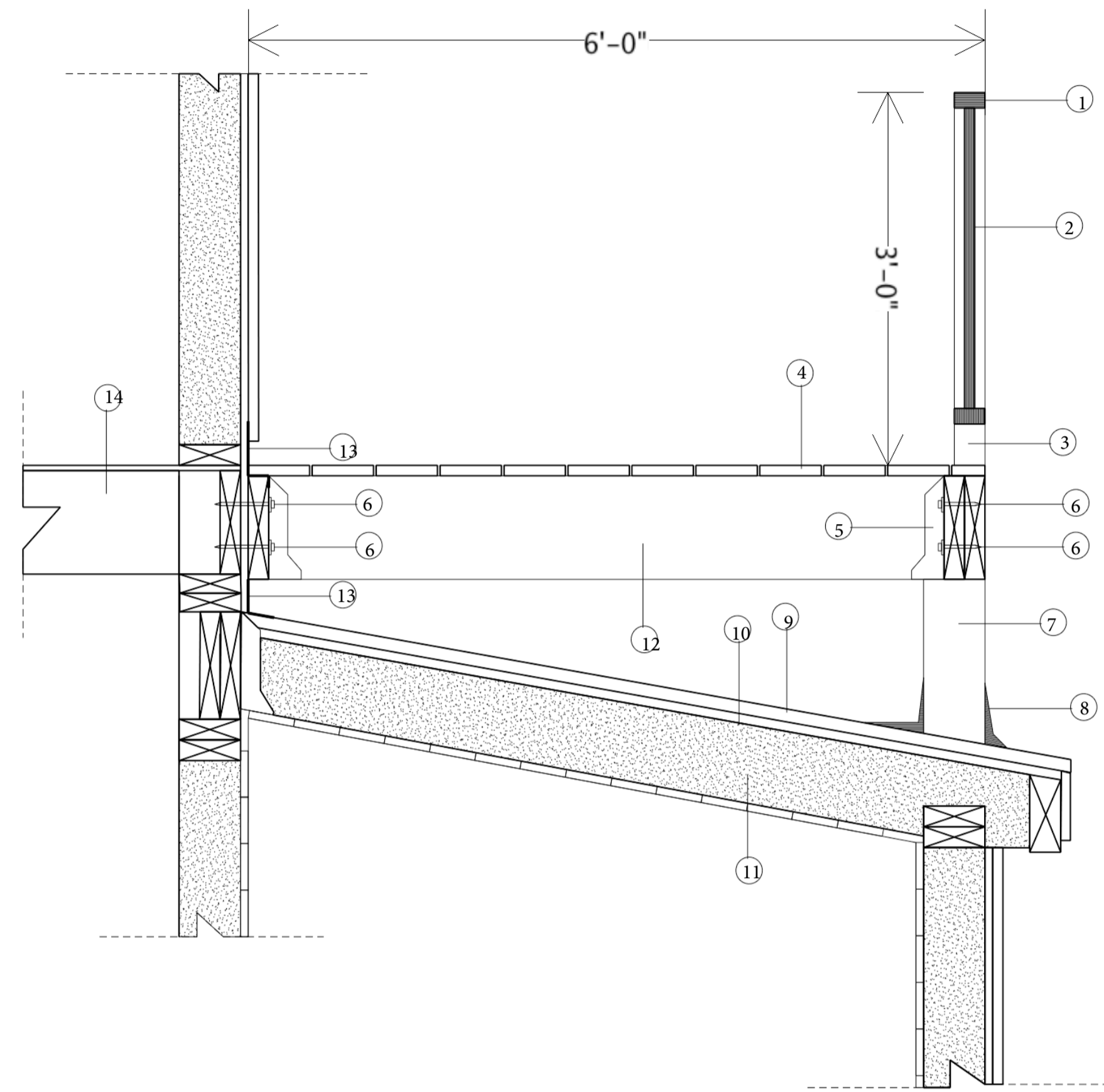
Section Detail- Second Floor Deck and Bathroom Ceiling 1" = 1'-0"
