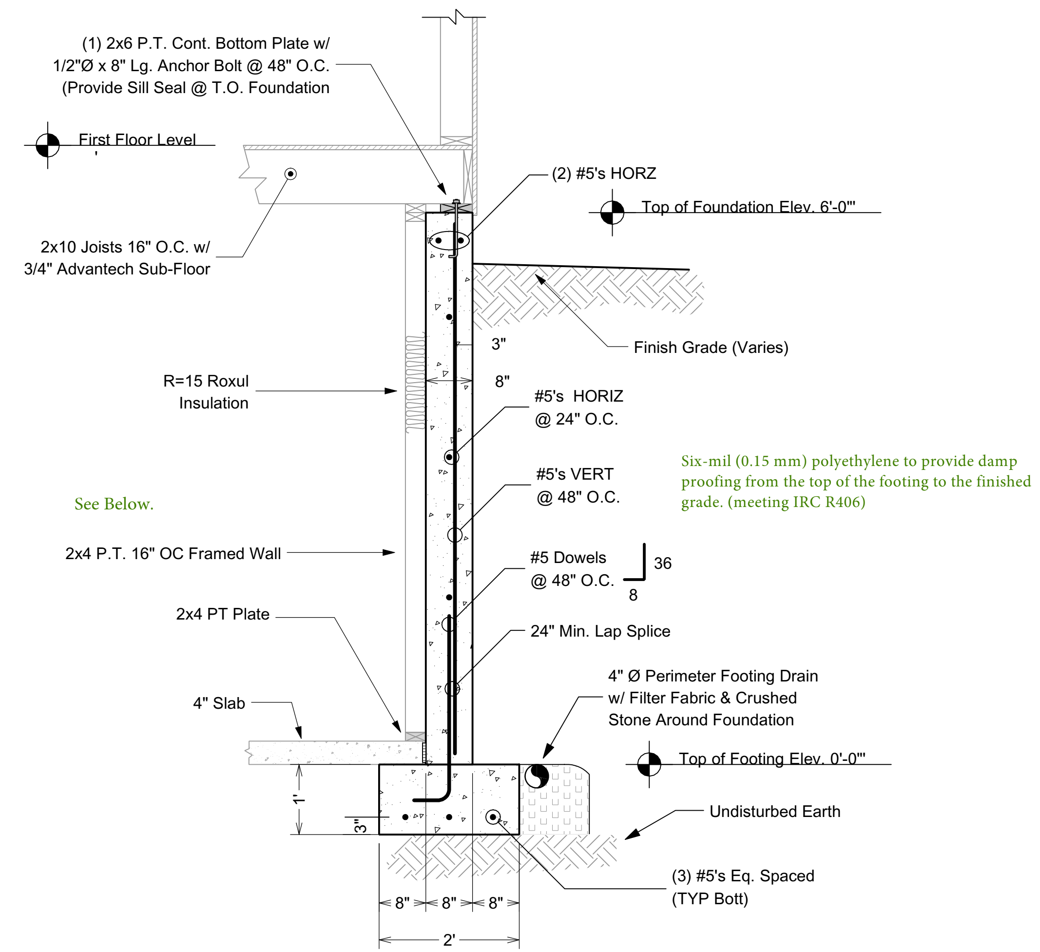
8" FOUNDATION DETAIL Scale: 3/4"=1'
