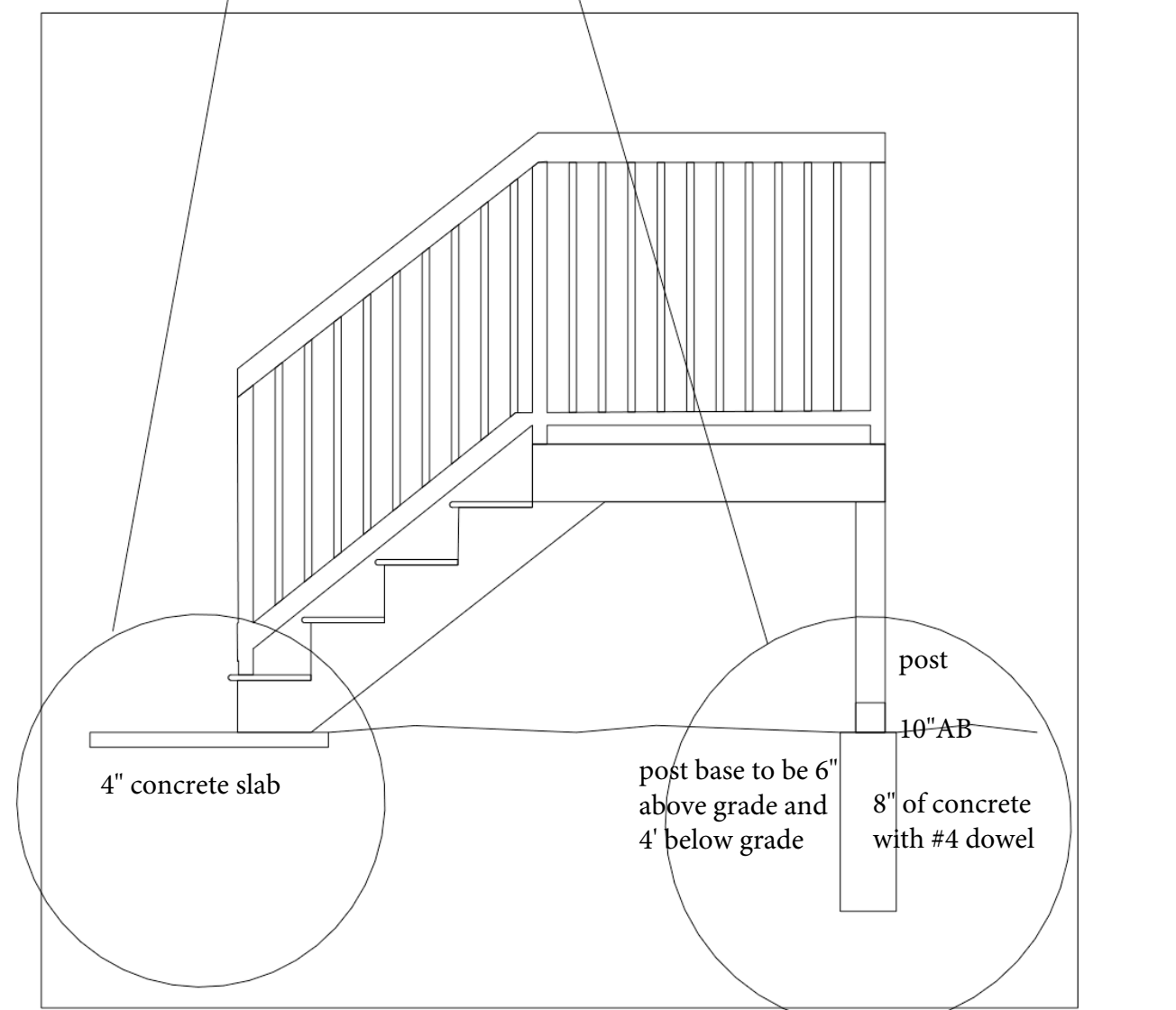
Exterior Stair Footing Detail 1/2"=1'-0"
