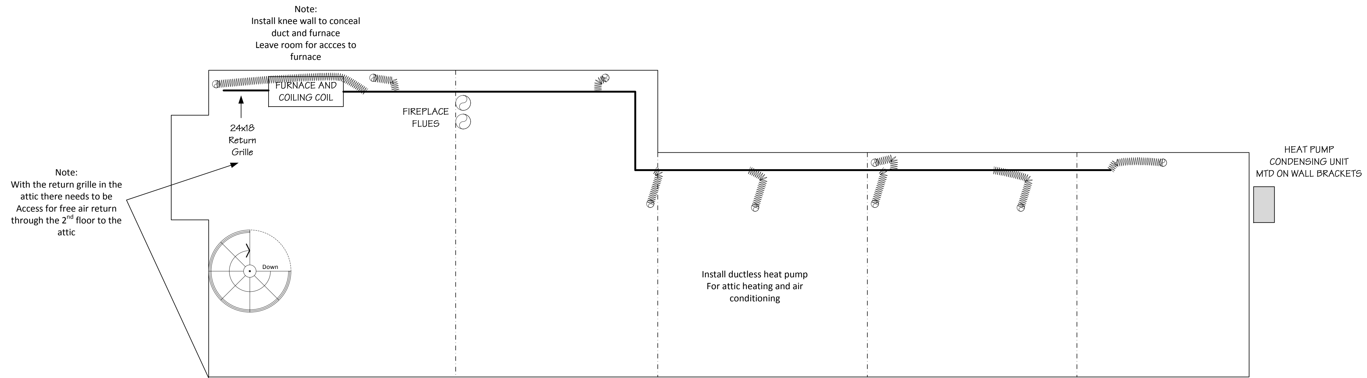
ATTIC FLOOR PLAN
