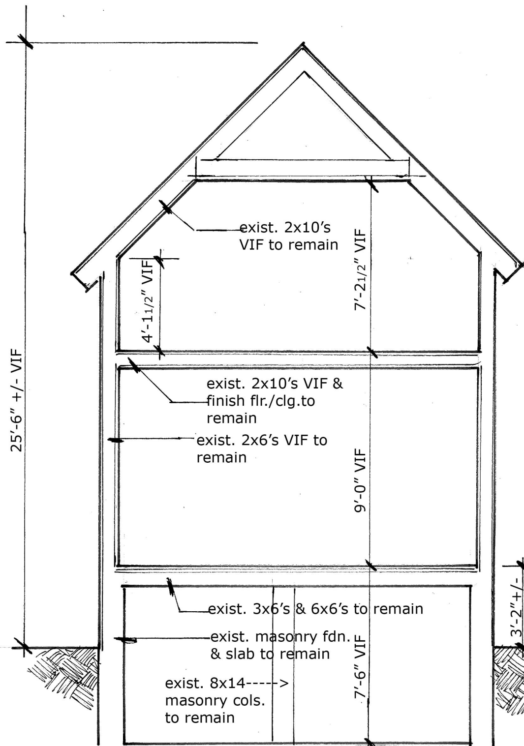
① Existing & Proposed Building Section 1/4"=1'-0" (no change)
