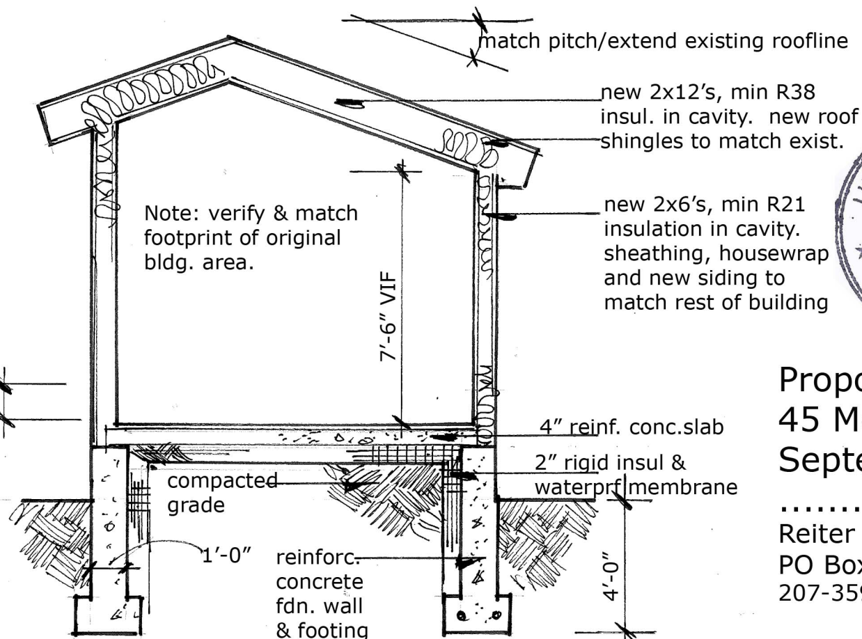
② Proposed Building Section @ Rear 1/4"=1'-0"
