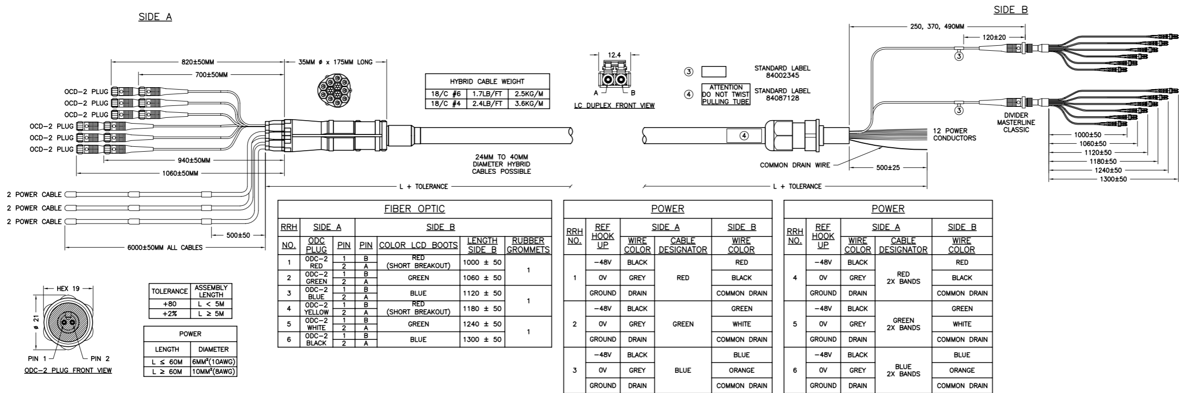
1 MLE HYBRID CABLE (6 POWER/12 FIBER) A-3 NTS
