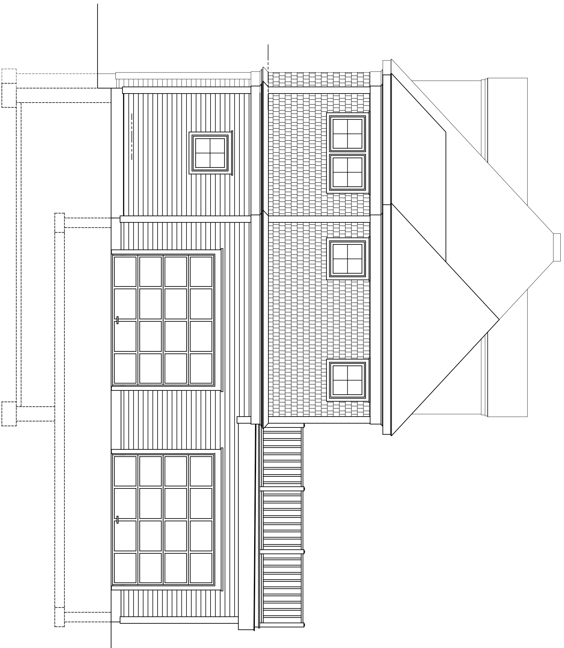
REAR ELEVATION
