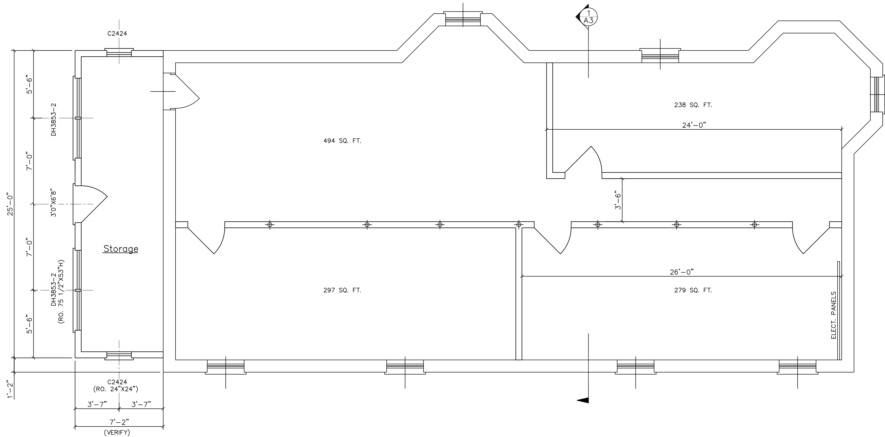
FLOOR PLAN-BASEMENT
