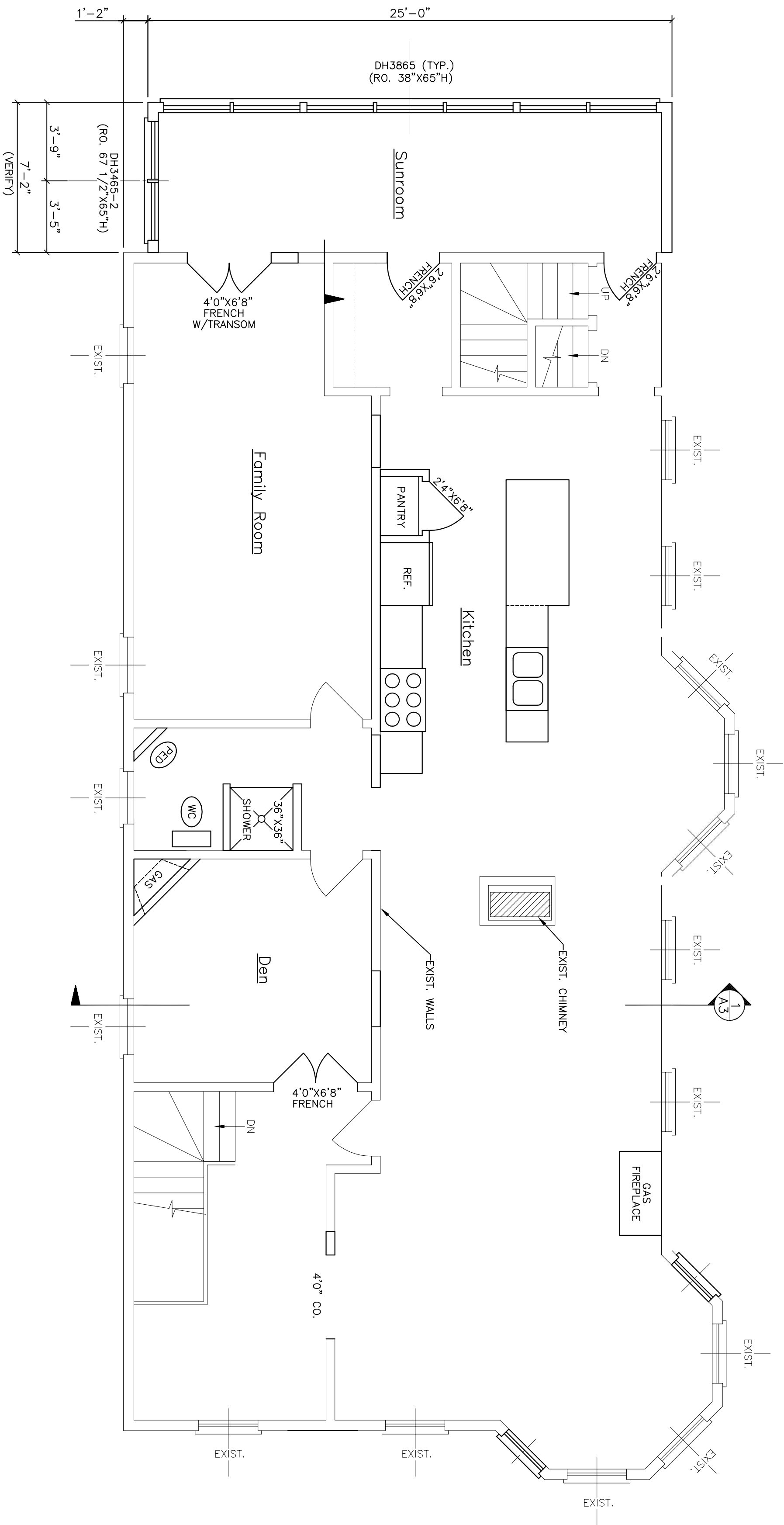
FLOOR PLAN—THIRD FLOOR
