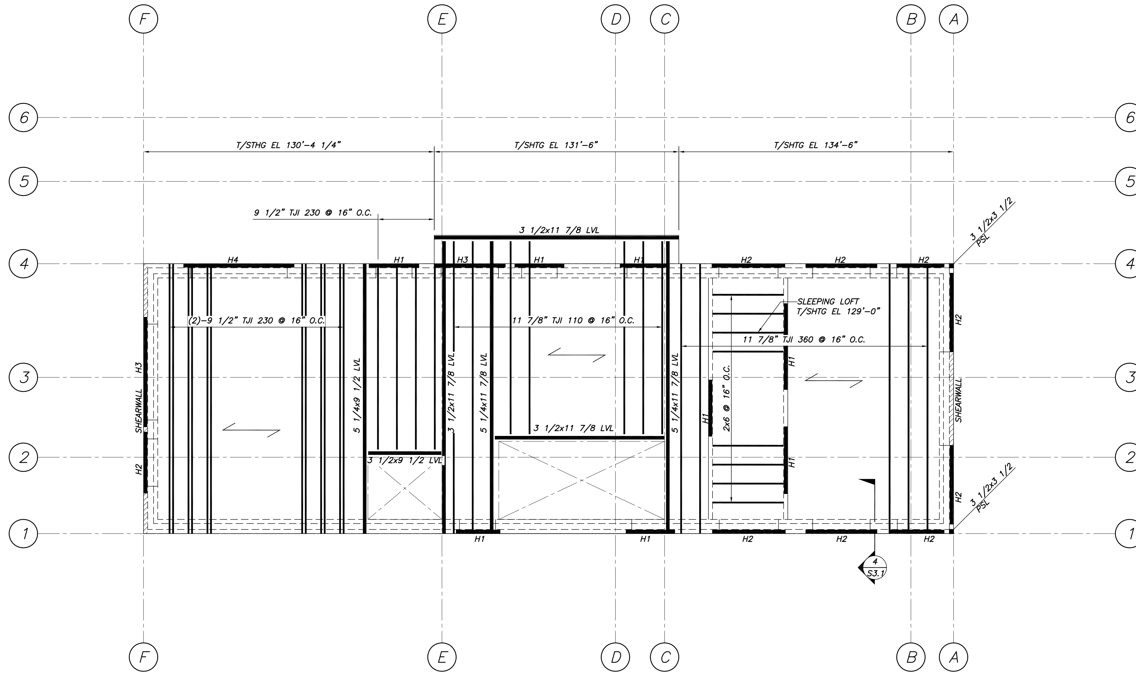
4TH FLOOR FRAMING PLAN 1/4"=1'-0"
