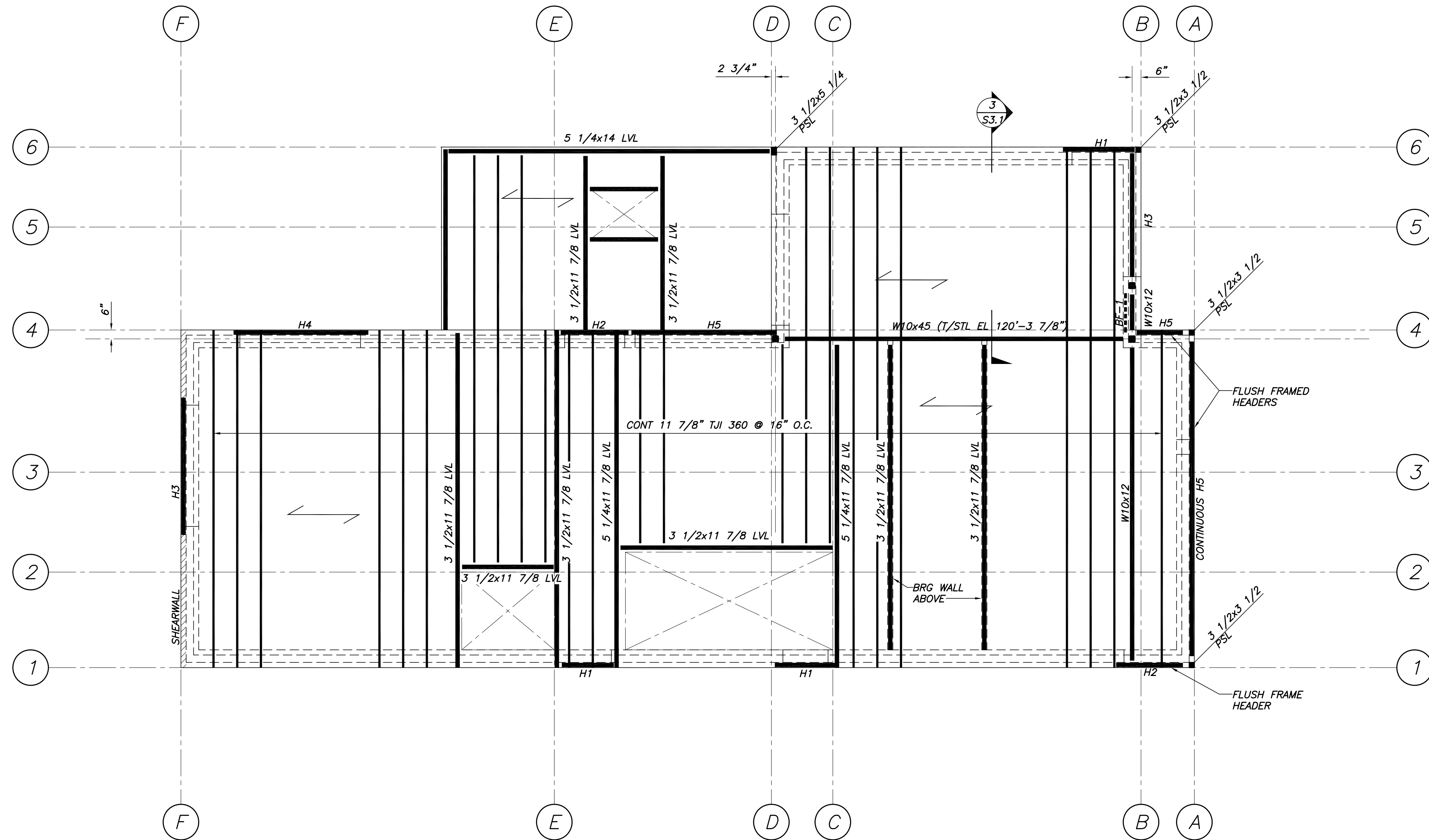
3RD FLOOR FRAMING PLAN 1/4"=1'-0"
