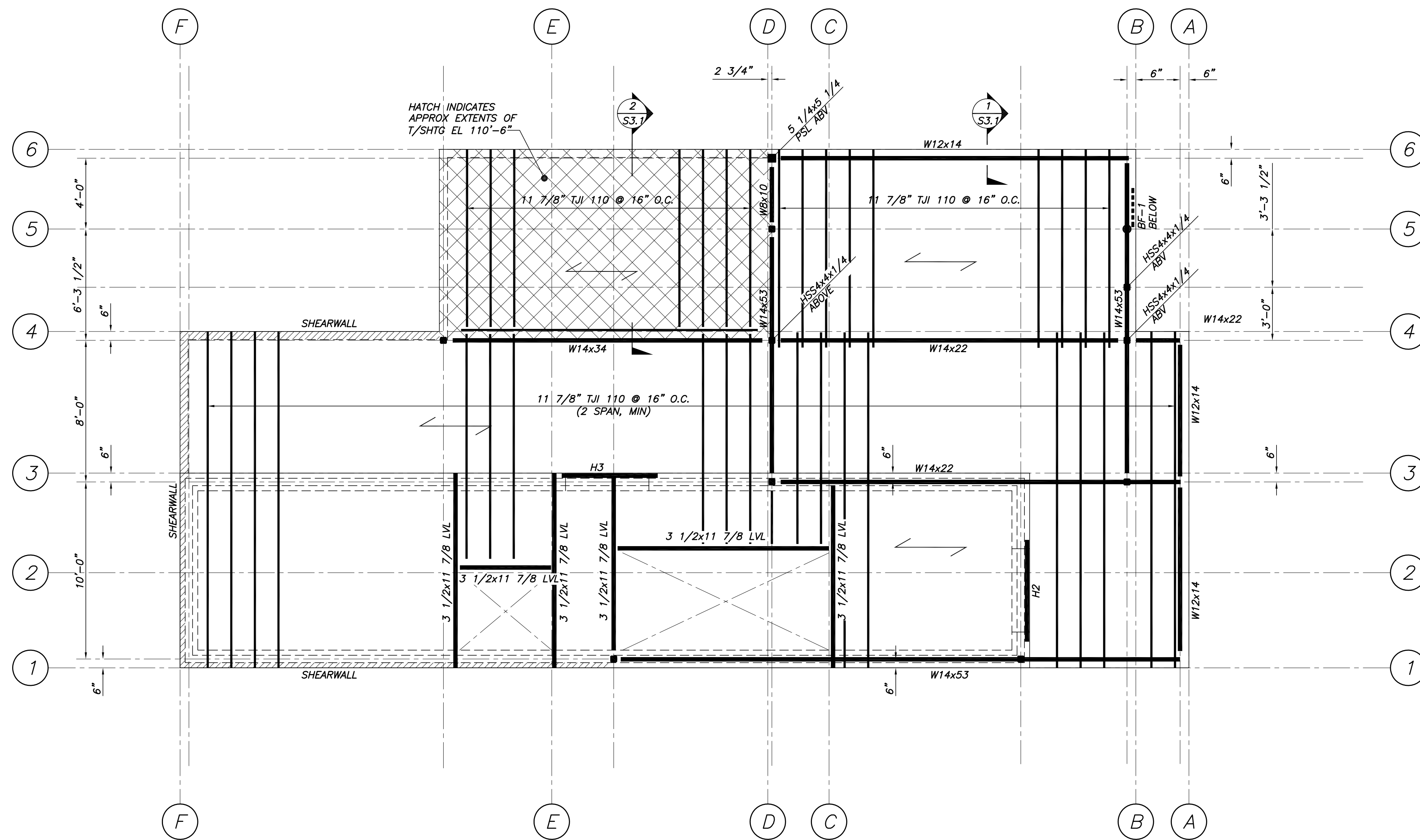
2ND FLOOR FRAMING PLAN 1/4"=1'-0"
