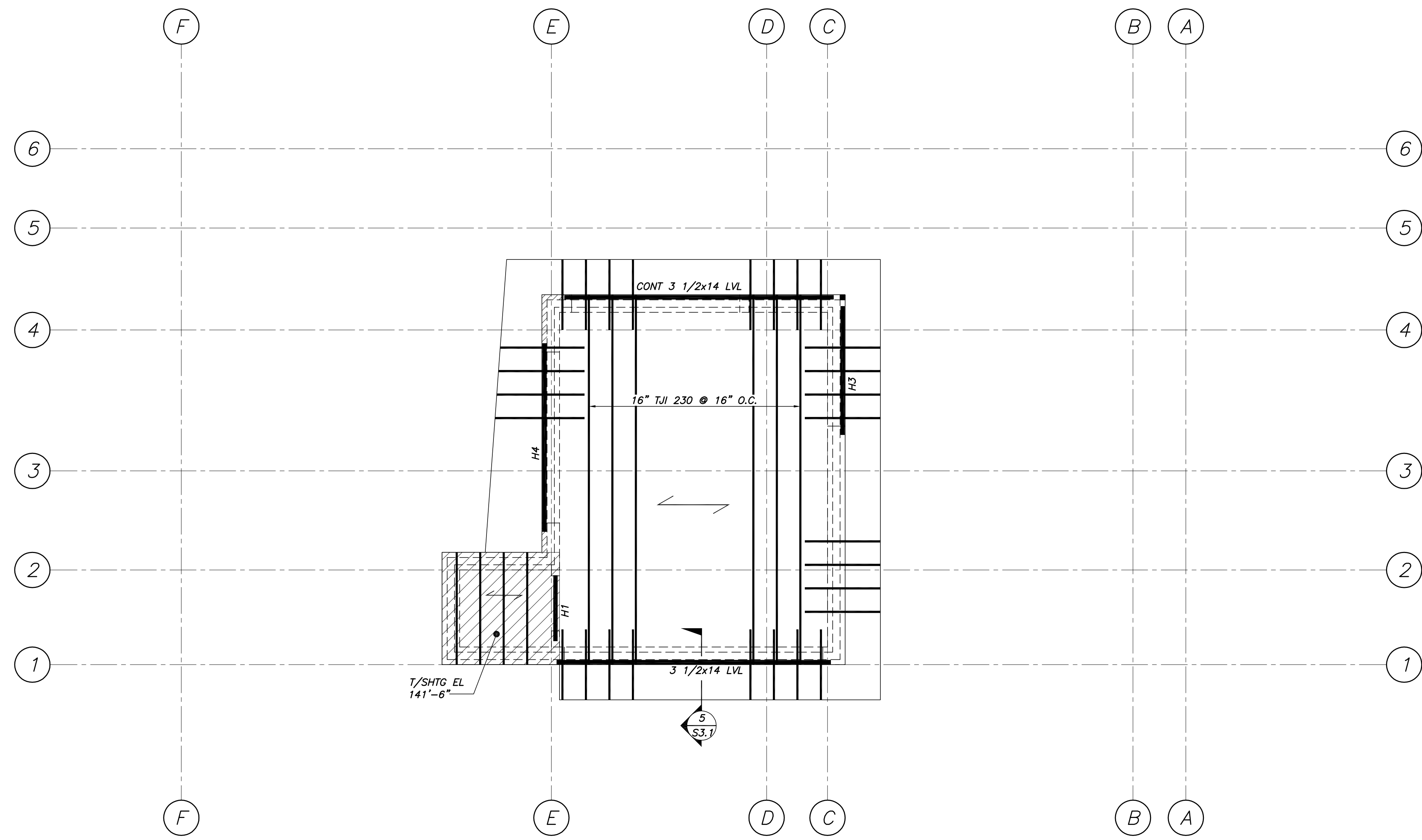
TOWER ROOF FRAMING PLAN 1/4"=1'-0"
