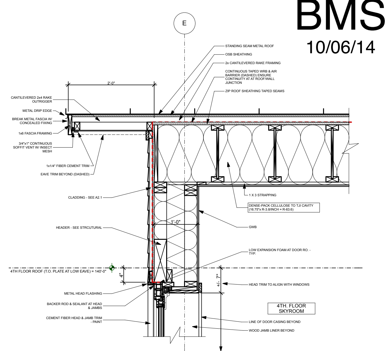
11 4TH. FLOOR RAKE - TYPICAL SCALE: 3/4" = 1'-0"
