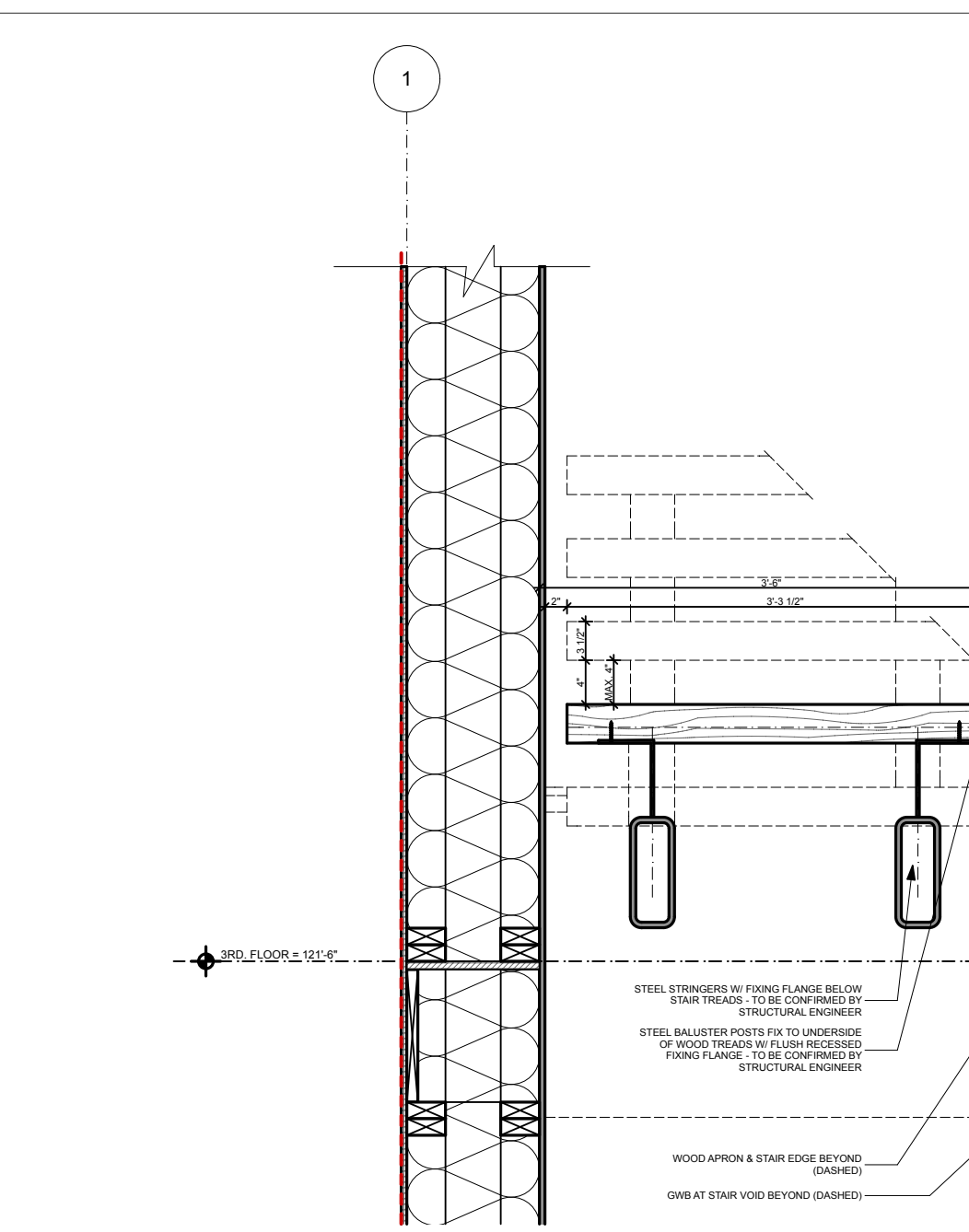
12 STAIR BALUSTRADE & BUILT-IN SHELF AT 3RD. FLOOR STAIR VOID SCALE: 3/4" = 1'-0"
