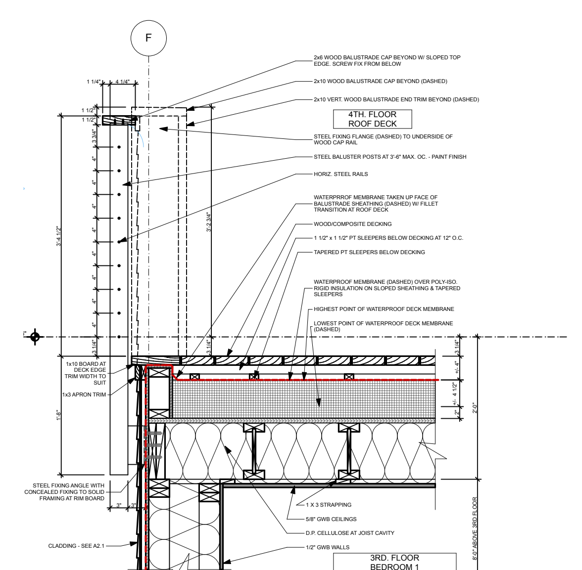
9 4TH FL. DECK - CABLE BALUSTRADE SCALE: 3/4" = 1'-0"
