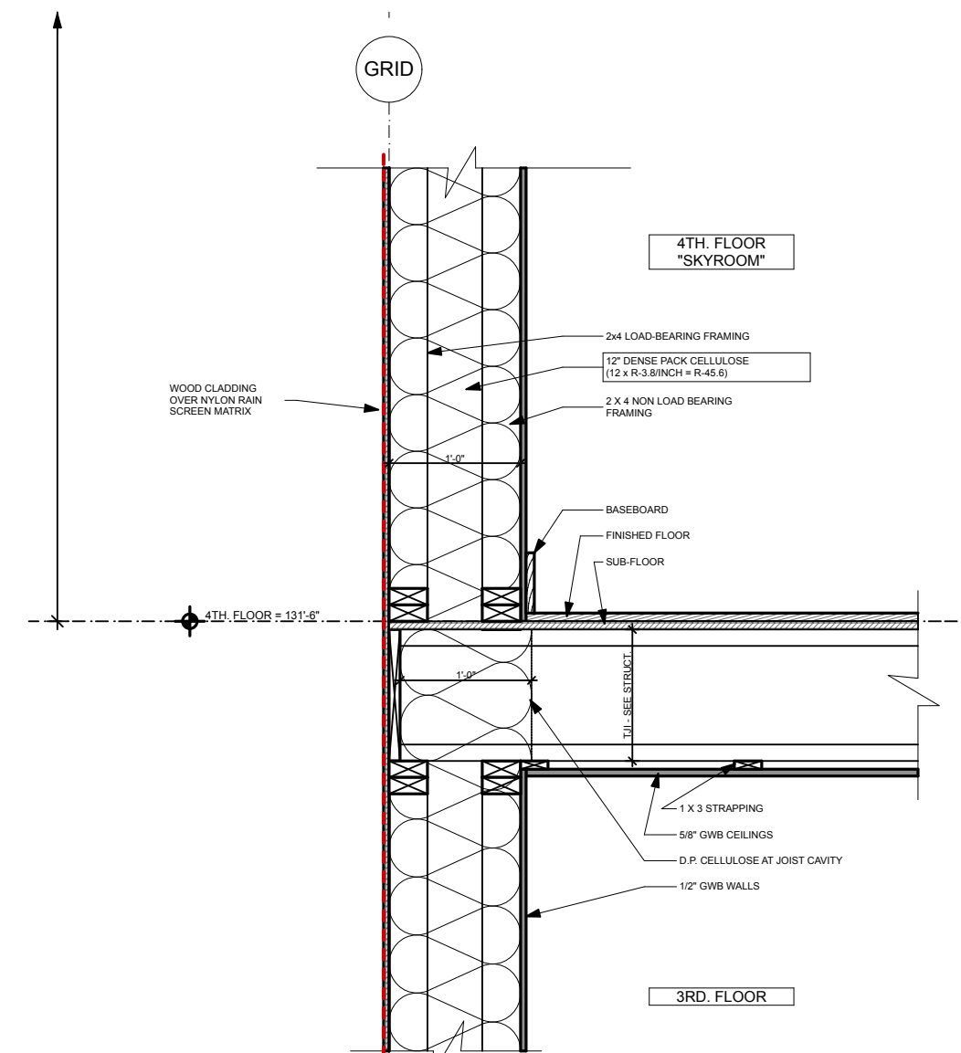
1 4TH. FLOOR RIM - TYPICAL SCALE: 3/4" = 1'-0"
