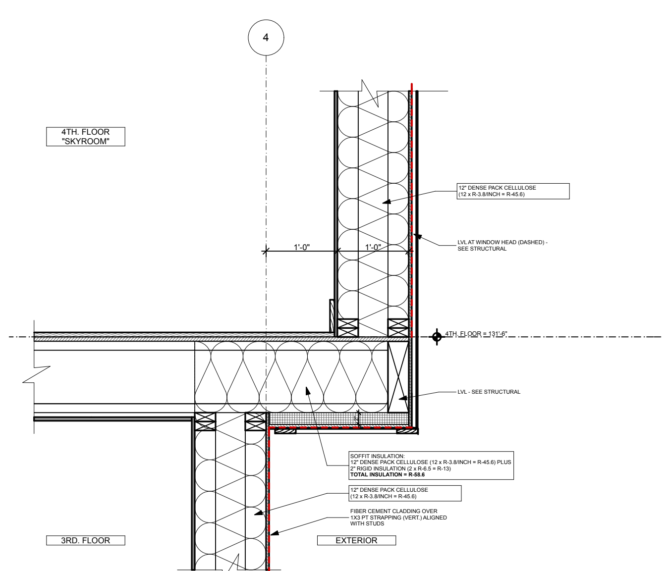
3 4TH. FLOOR - AT OVERHANG SCALE: 3/4" = 1'-0"
