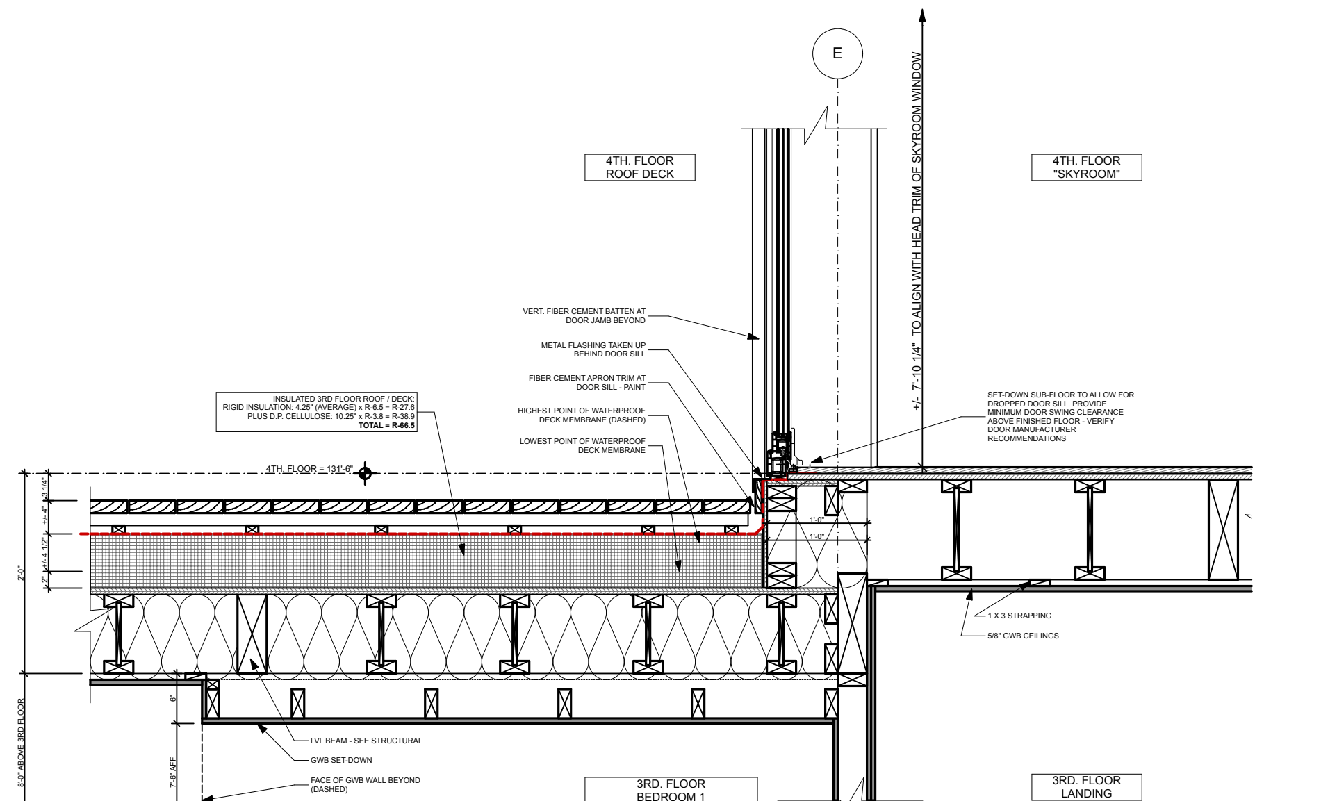
10 4TH FL. DECK AT SKYROOM DOOR SILL SCALE: 3/4" = 1'-0"
