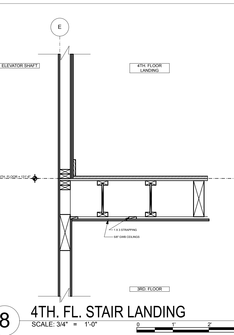
8 4TH. FL. STAIR LANDING SCALE: 3/4" = 1'-0"
