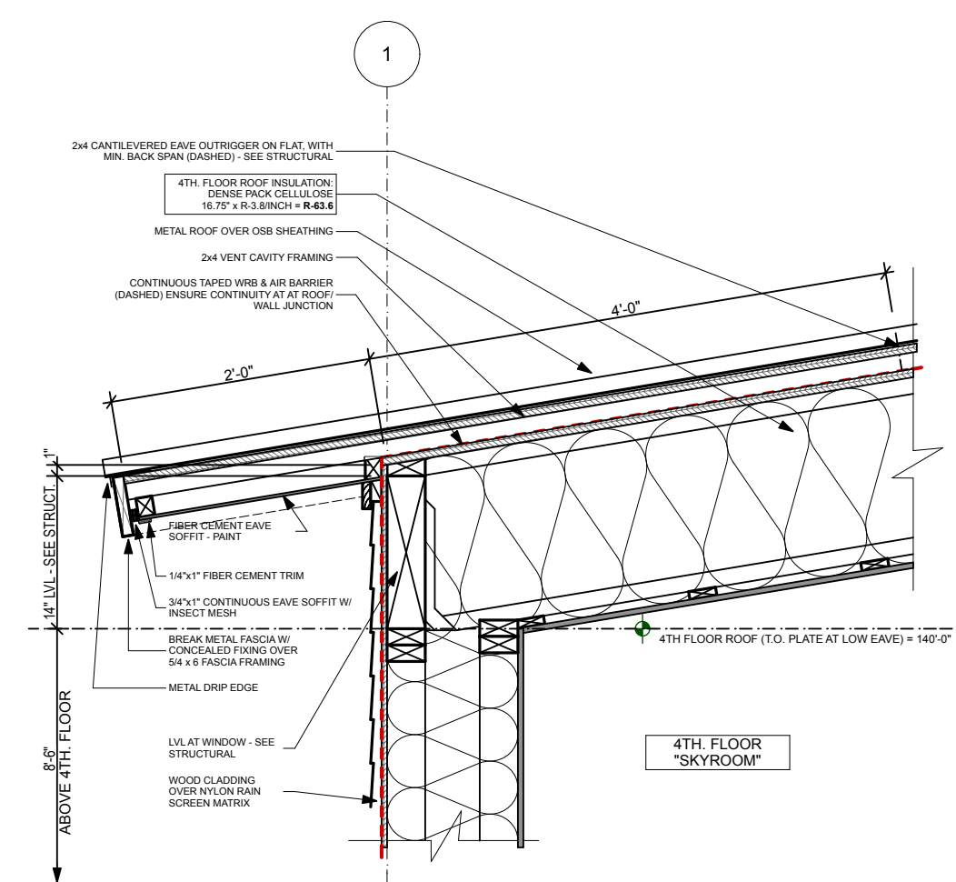
4 4TH. FLOOR EAVE - LOW - TYP. SCALE: 3/4" = 1'-0"
