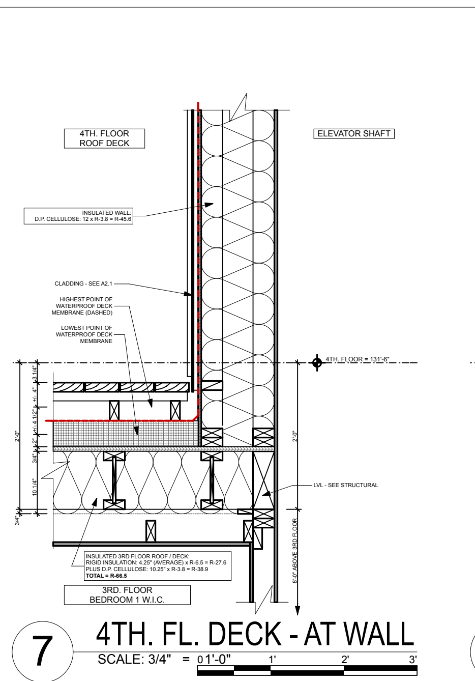
7 4TH. FL. DECK - AT WALL SCALE: 3/4" = 1'-0"
