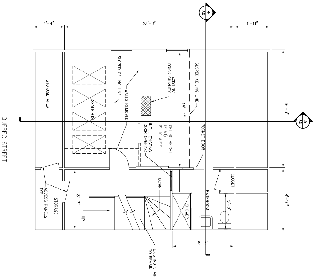
THIRD FLOOR PLAN 1/4" = 1'-0"
