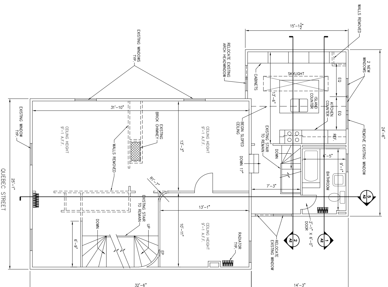
SECOND FLOOR PLAN 1/4" = 1'-0"
