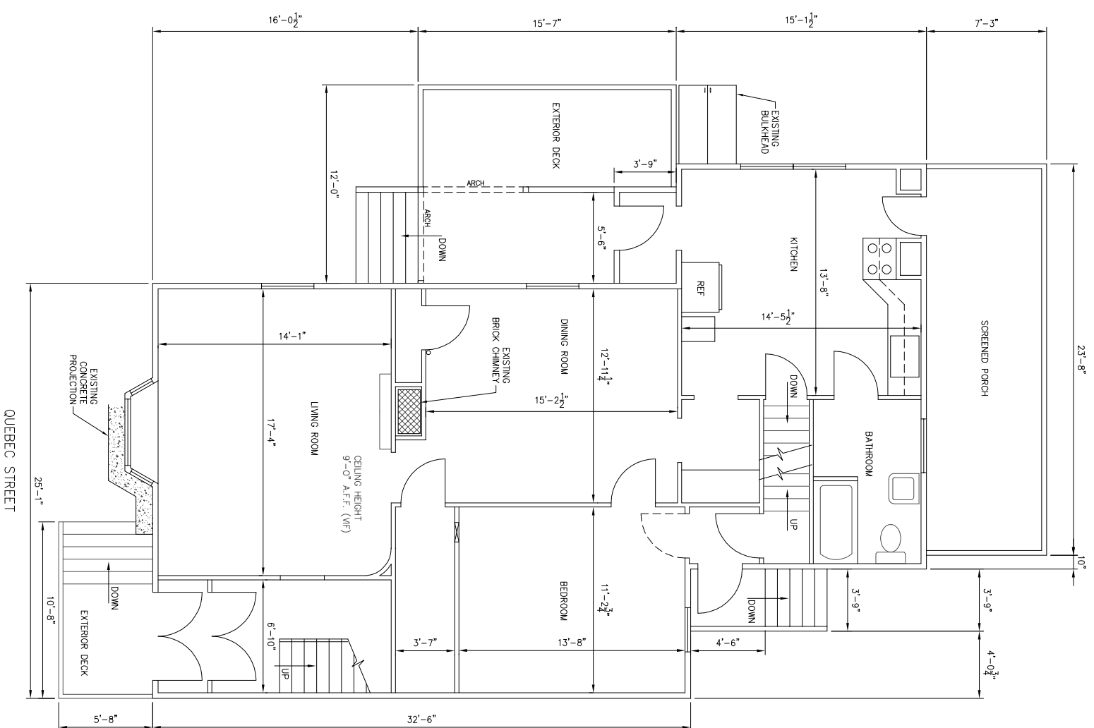
FIRST FLOOR PLAN 1/4" = 1'-0"
