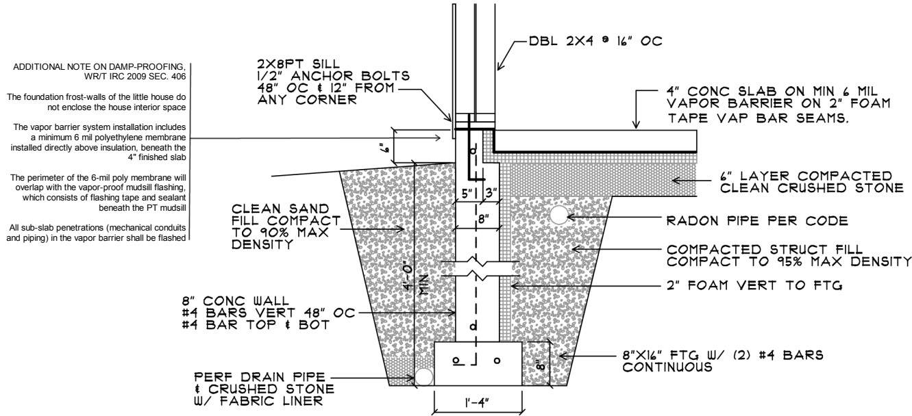
1 TYPICAL FOUNDATION WALL SK2
