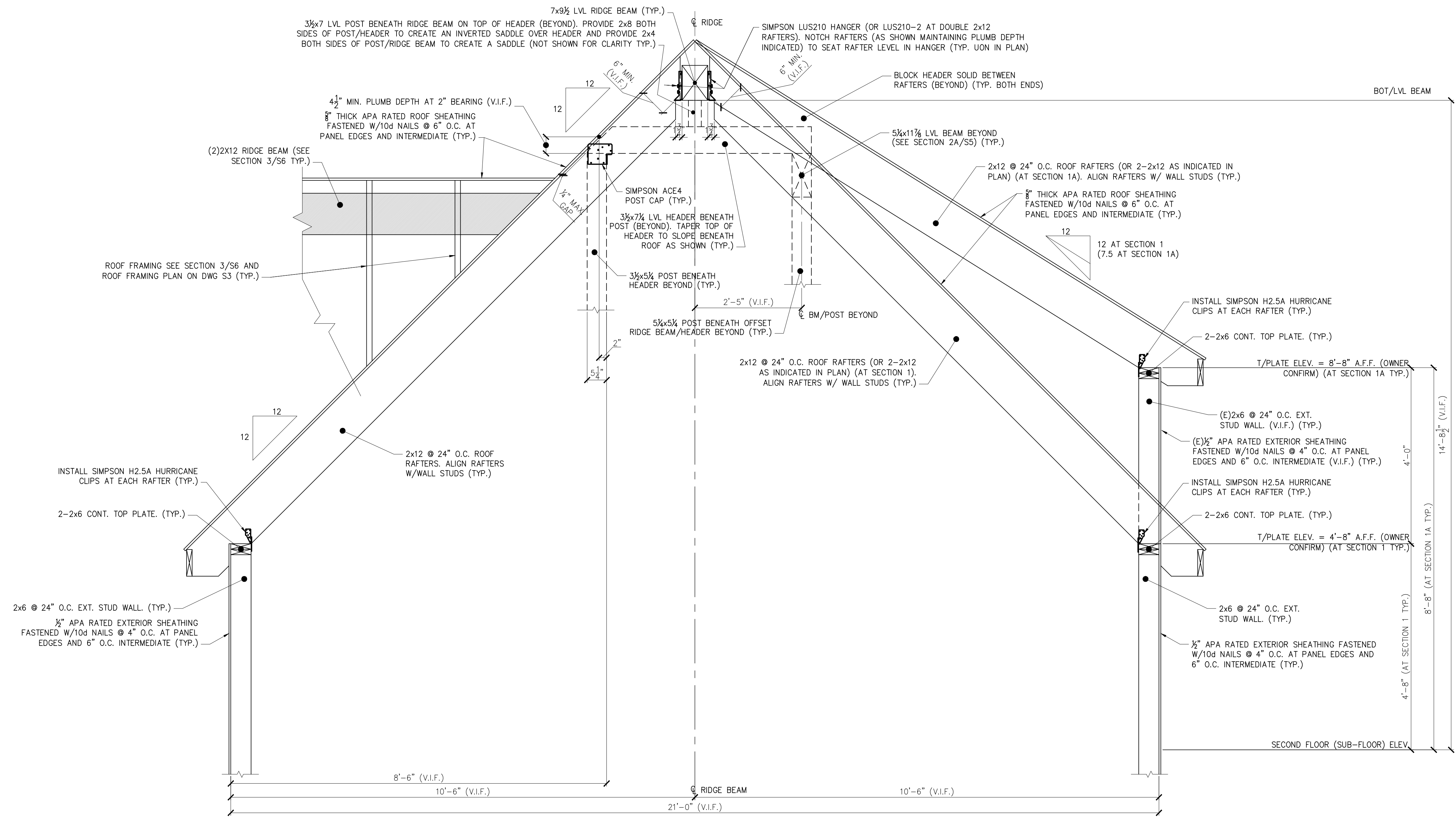
SECTION 1 1A S3 S3 3/4" = 1'-0"
