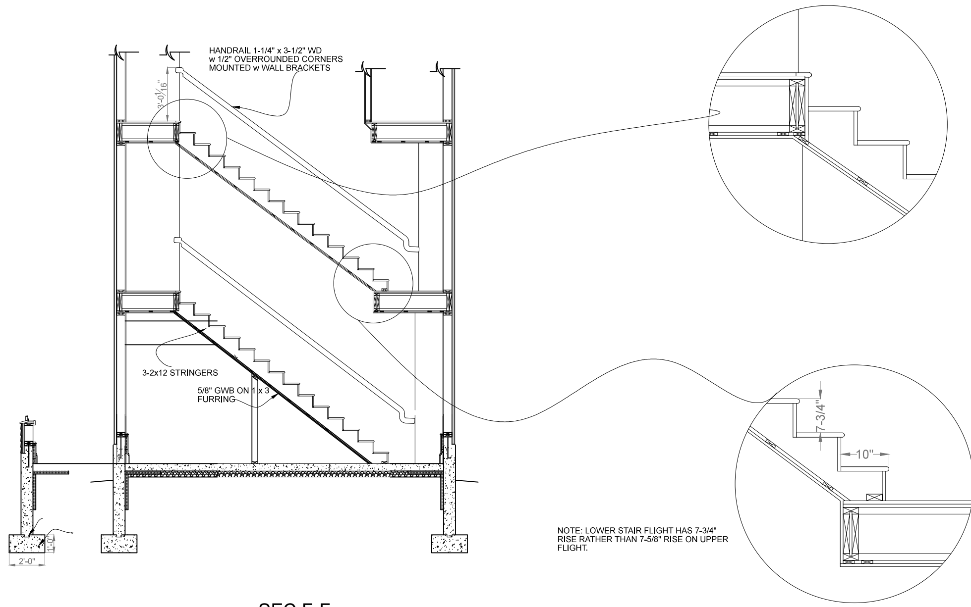
SEC F-F
