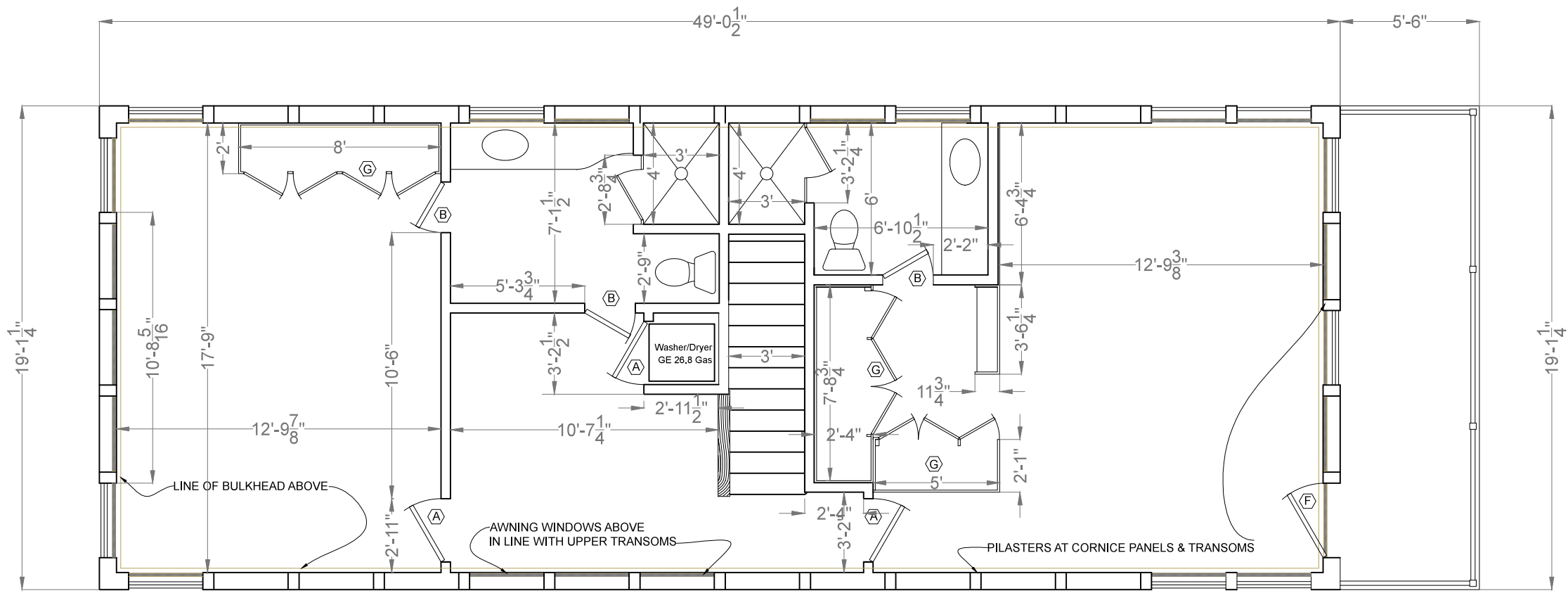
2nd FLOOR
