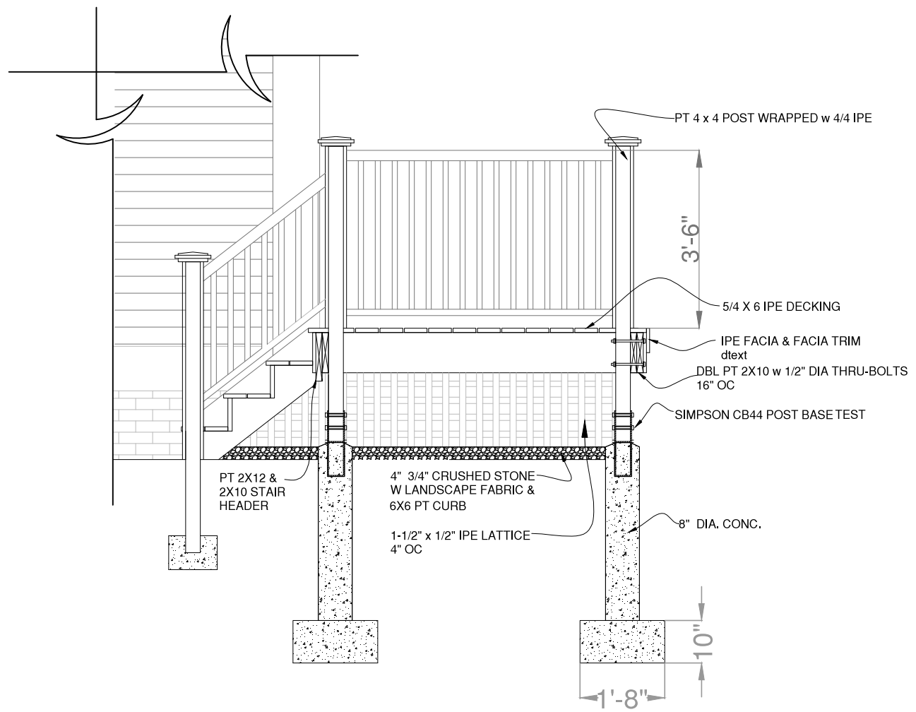
SEC E-E
