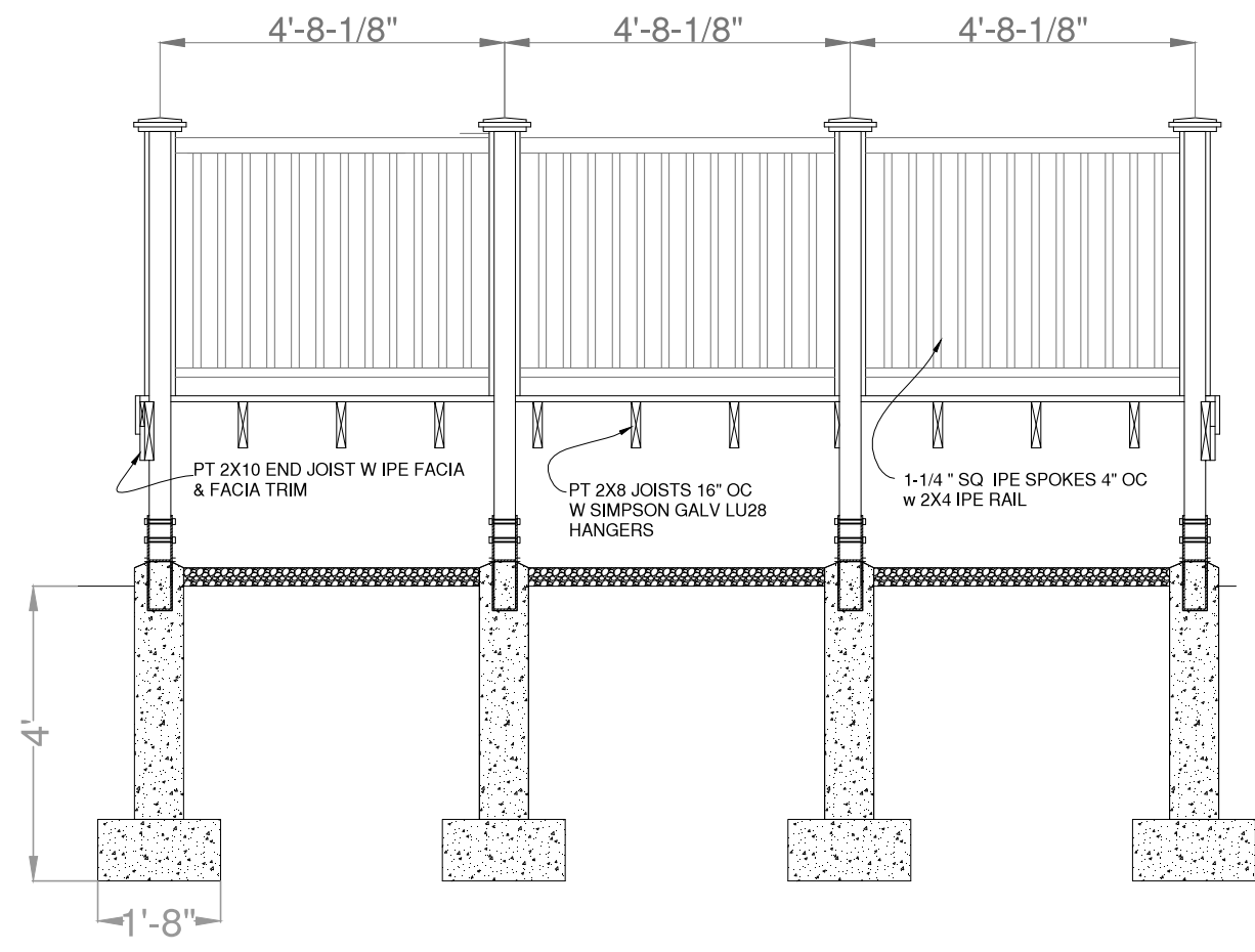
SEC C-C
