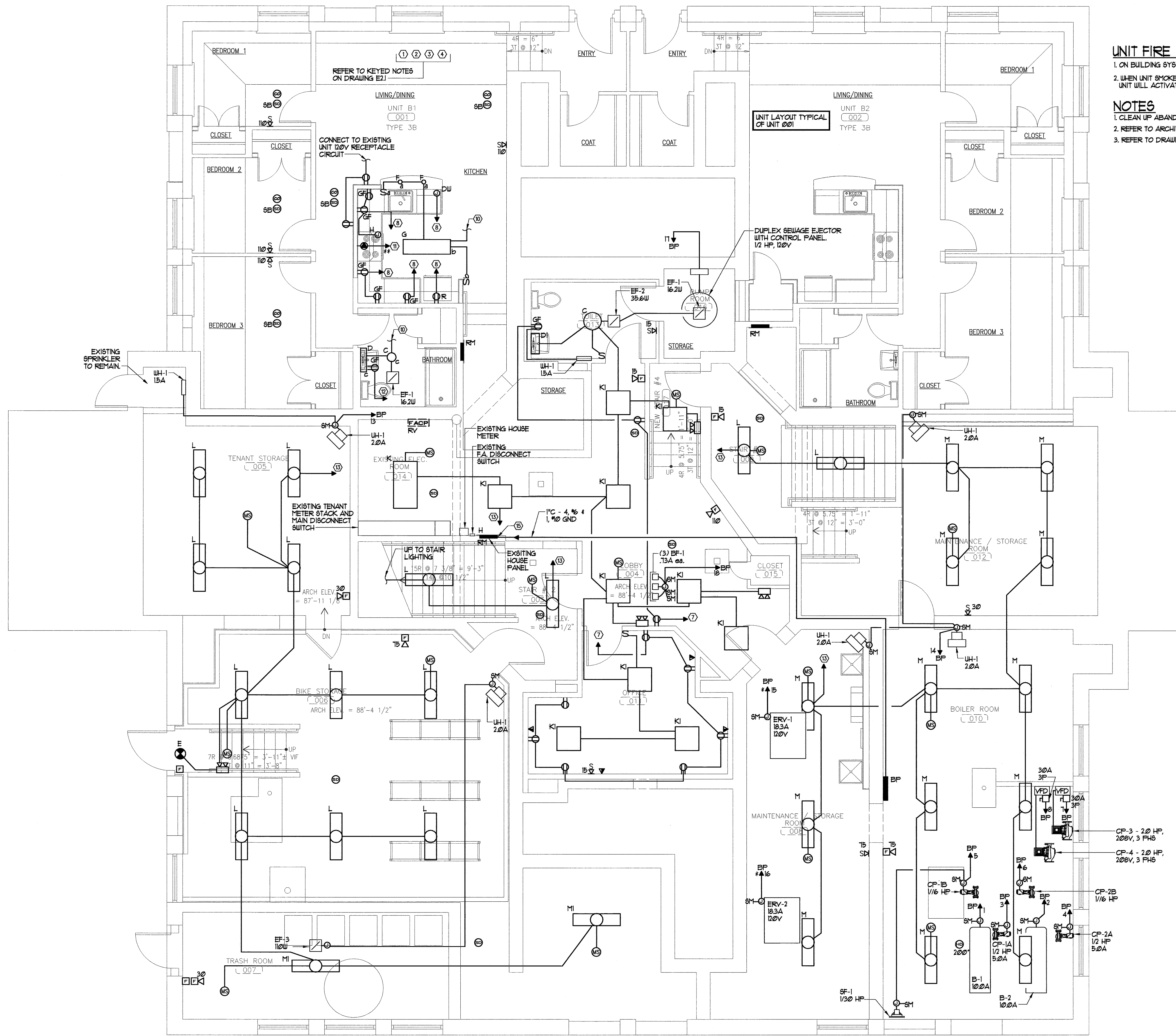
1 BASEMENT ELECTRICAL PLAN REFERENCED FROM:
