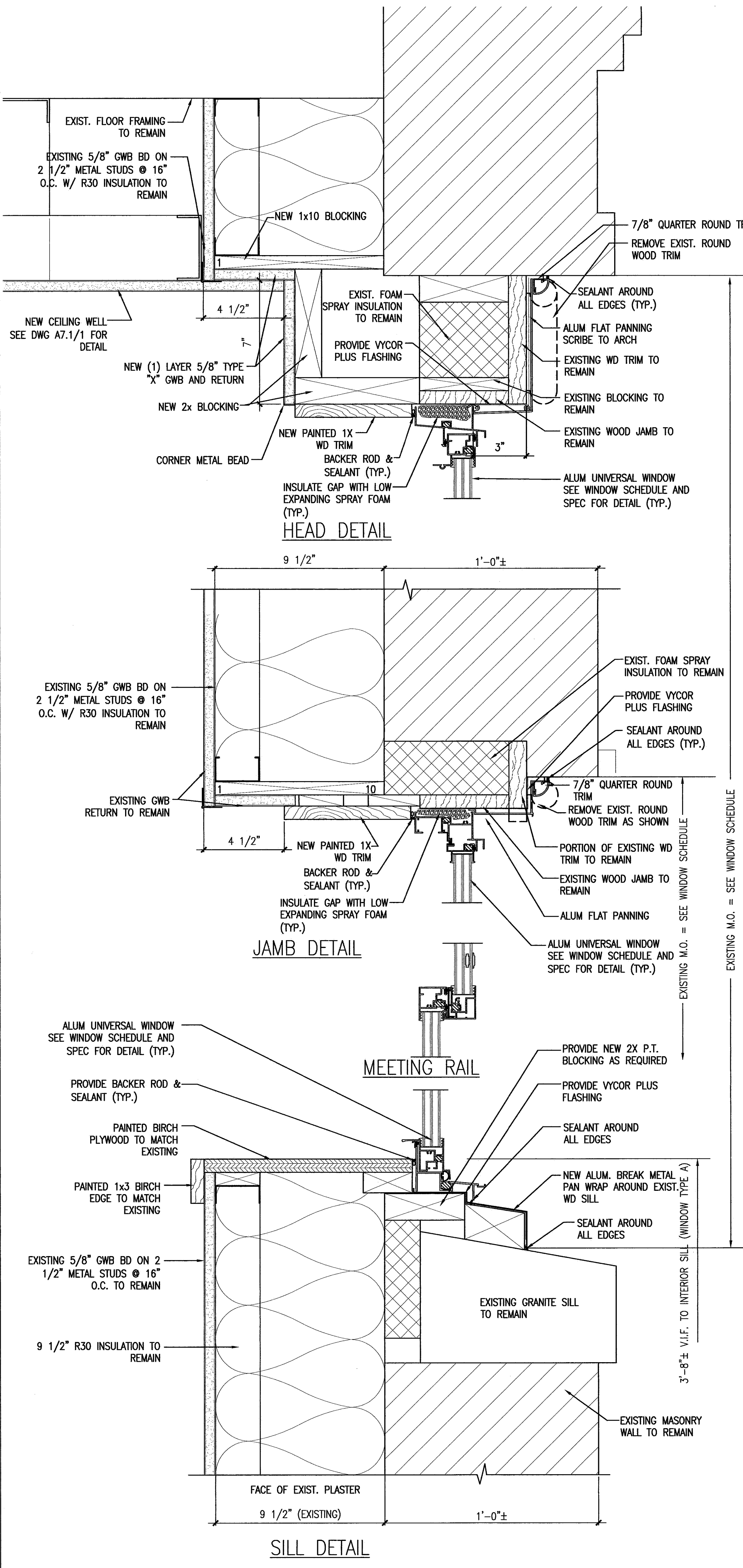
2 NEW WINDOW - SILL, JAMB AND HEAD DETAILS REFERENCED FROM: SCALE: 3" = 1'-0"
