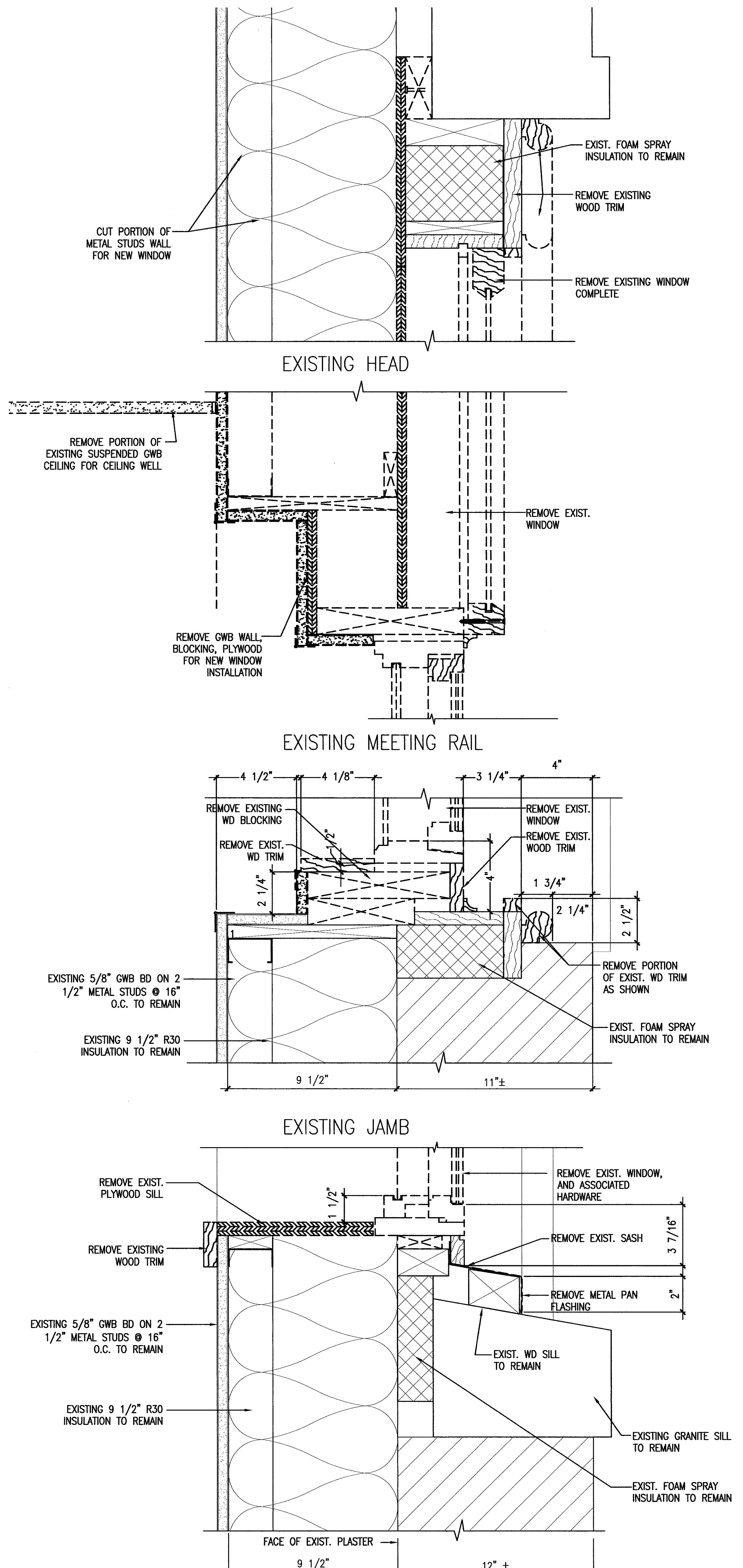
1 EXISTING WINDOW - SILL, JAMB AND HEAD DETAILS REFERENCED FROM: SCALE: 3" = 1'-0"
