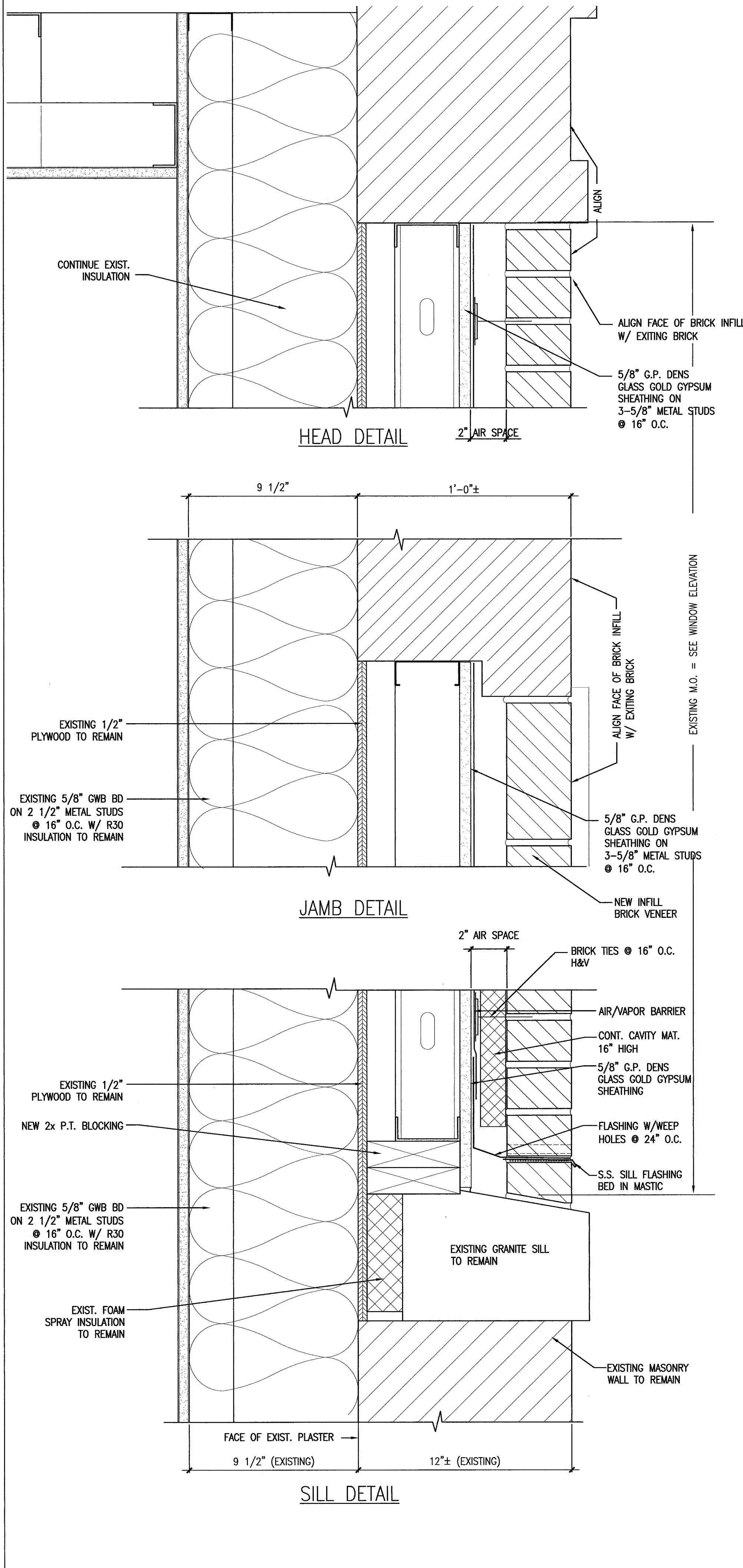
3 NEW INFILL BRICK VENEER - SILL, JAMB AND HEAD DETAILS REFERENCED FROM: SCALE: 3" = 1'-0"
