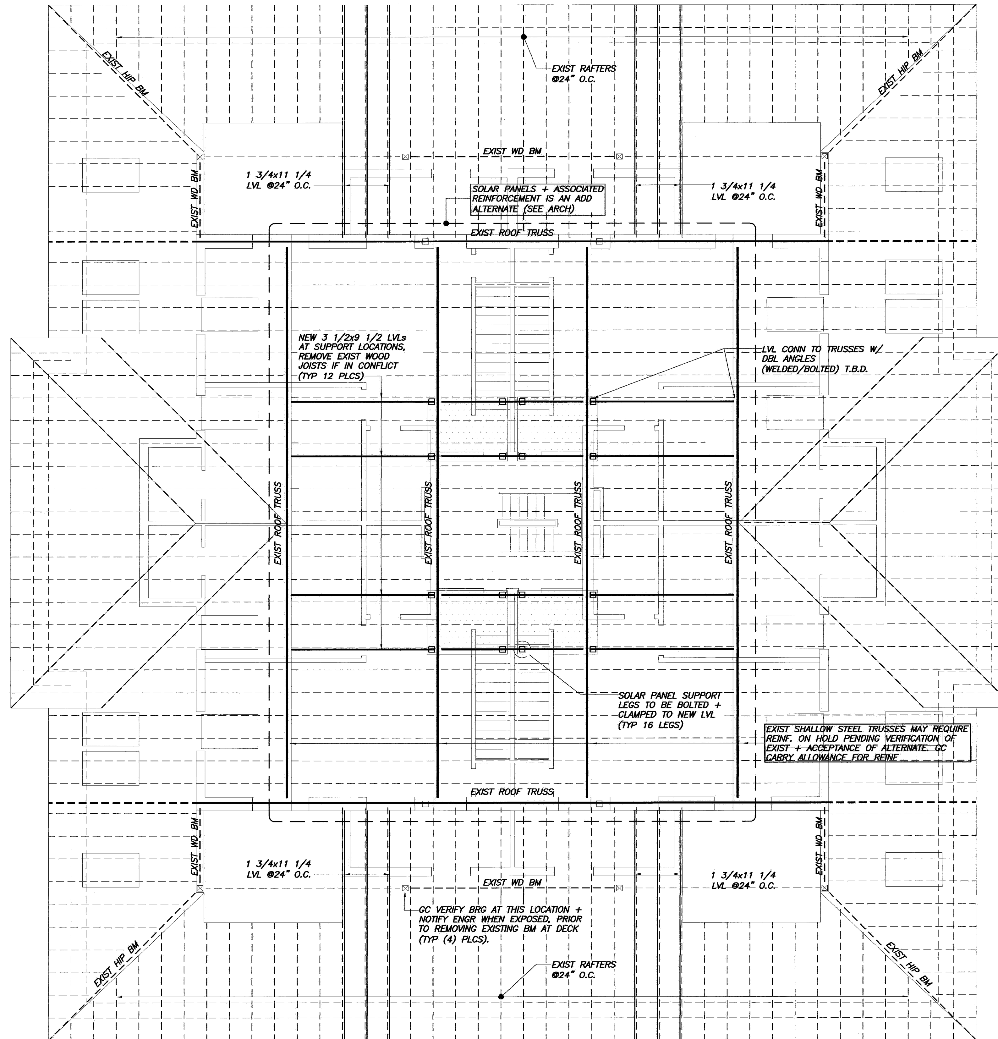
ROOF FRAMING PLAN 3/32"=1'-0"
