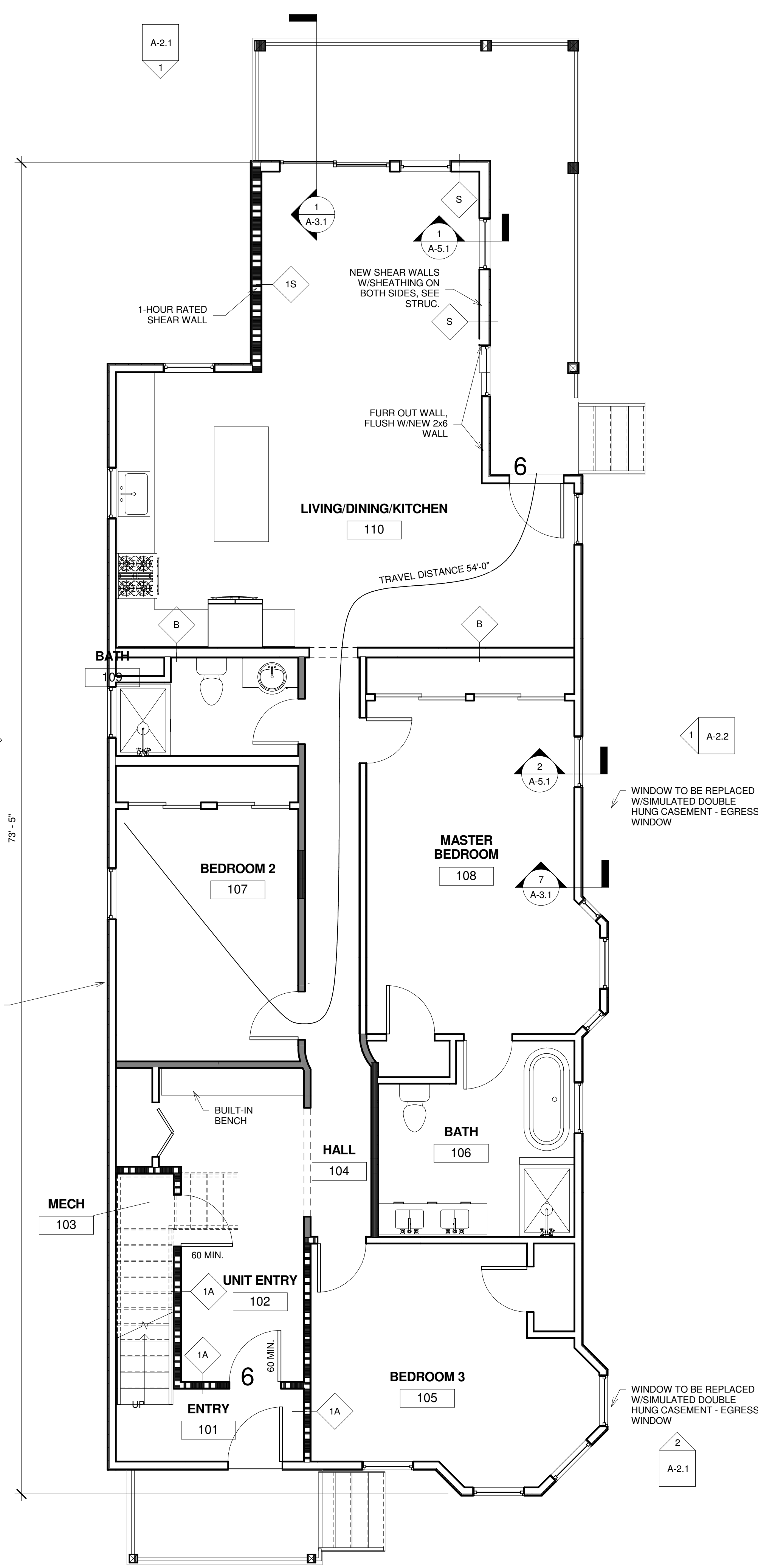
1 First Floor Life Safety Plan 1/4" = 1'-0"
