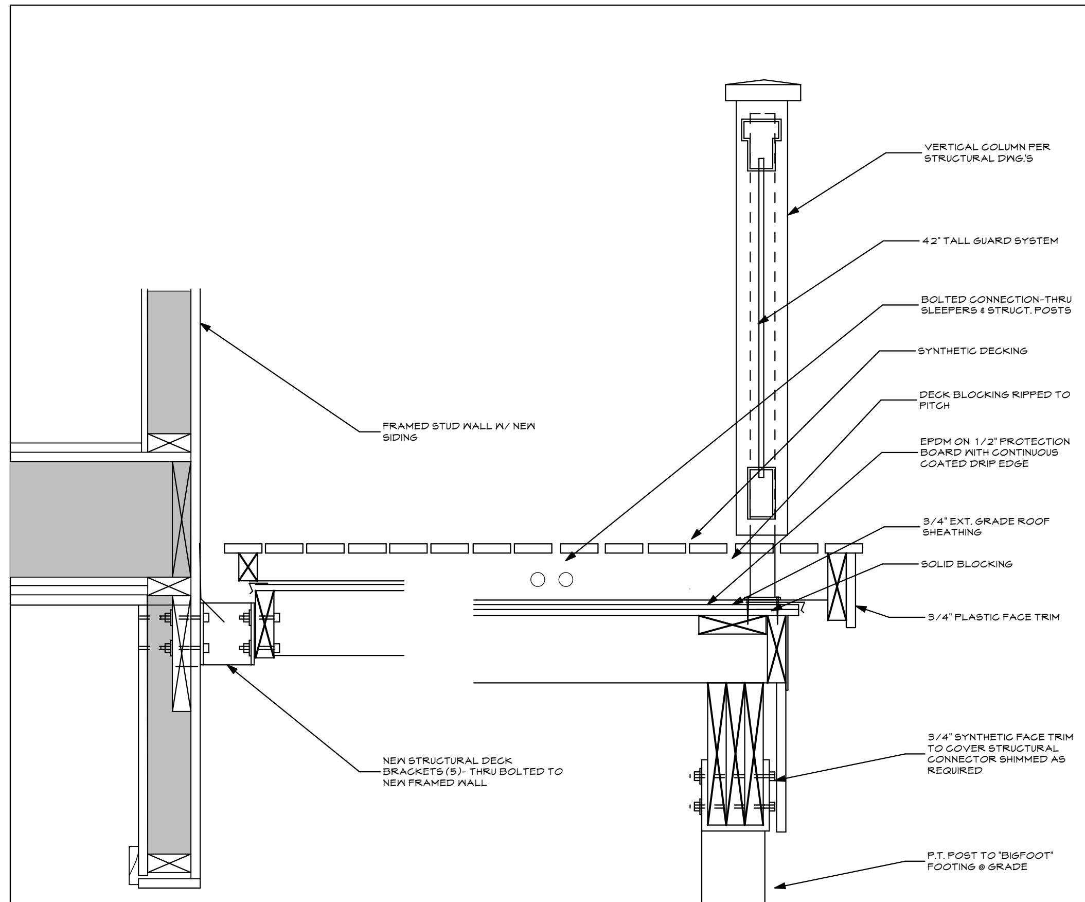
1. DECK TO WALL DETAIL
