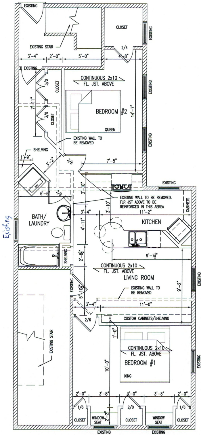
FLOOR PLAN 1/4" = 1'-0"
