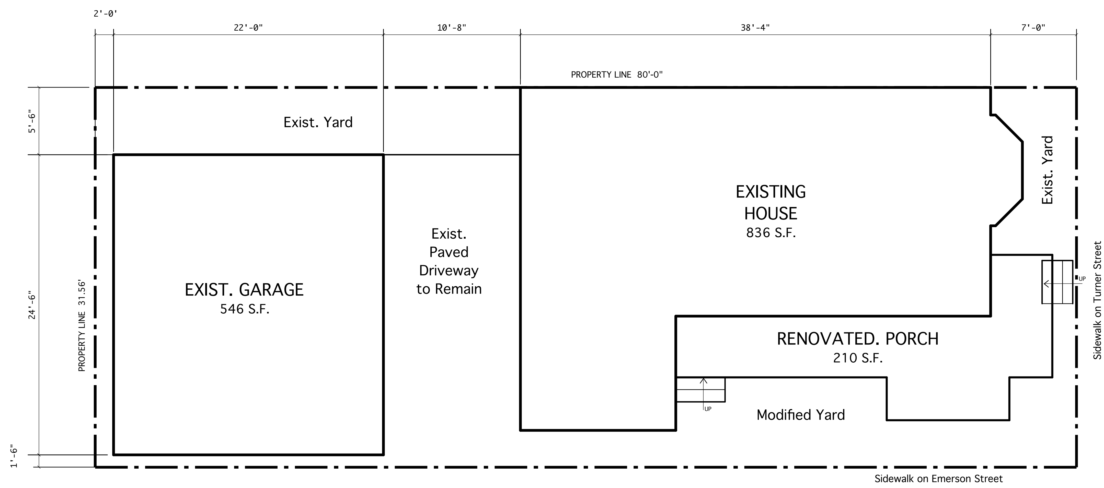
EXISTING PLOT PLAN
