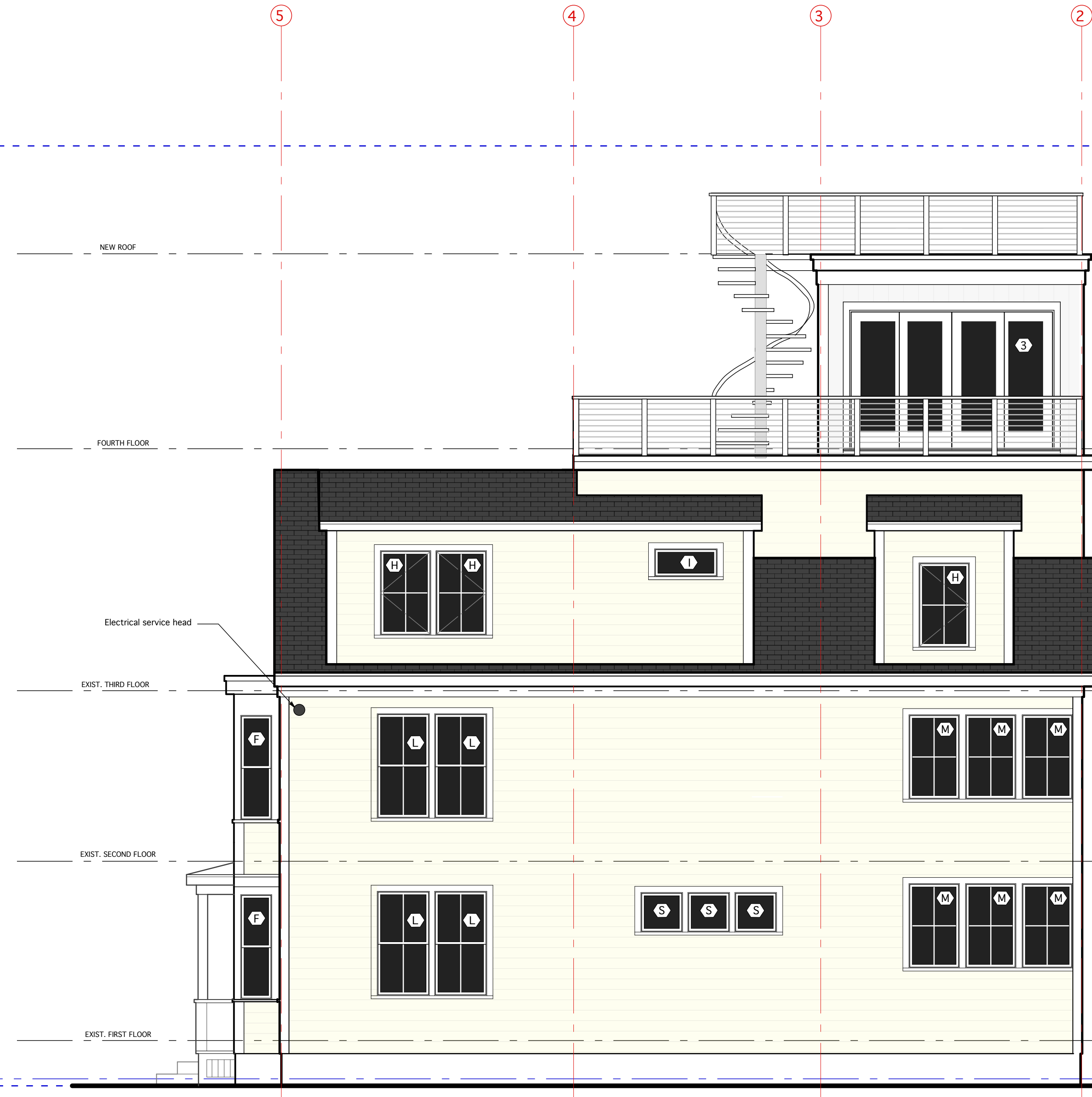
SCHEMATIC ELEVATION - NORTH
