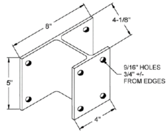
FIGURE 1—BRACKET DETAIL
