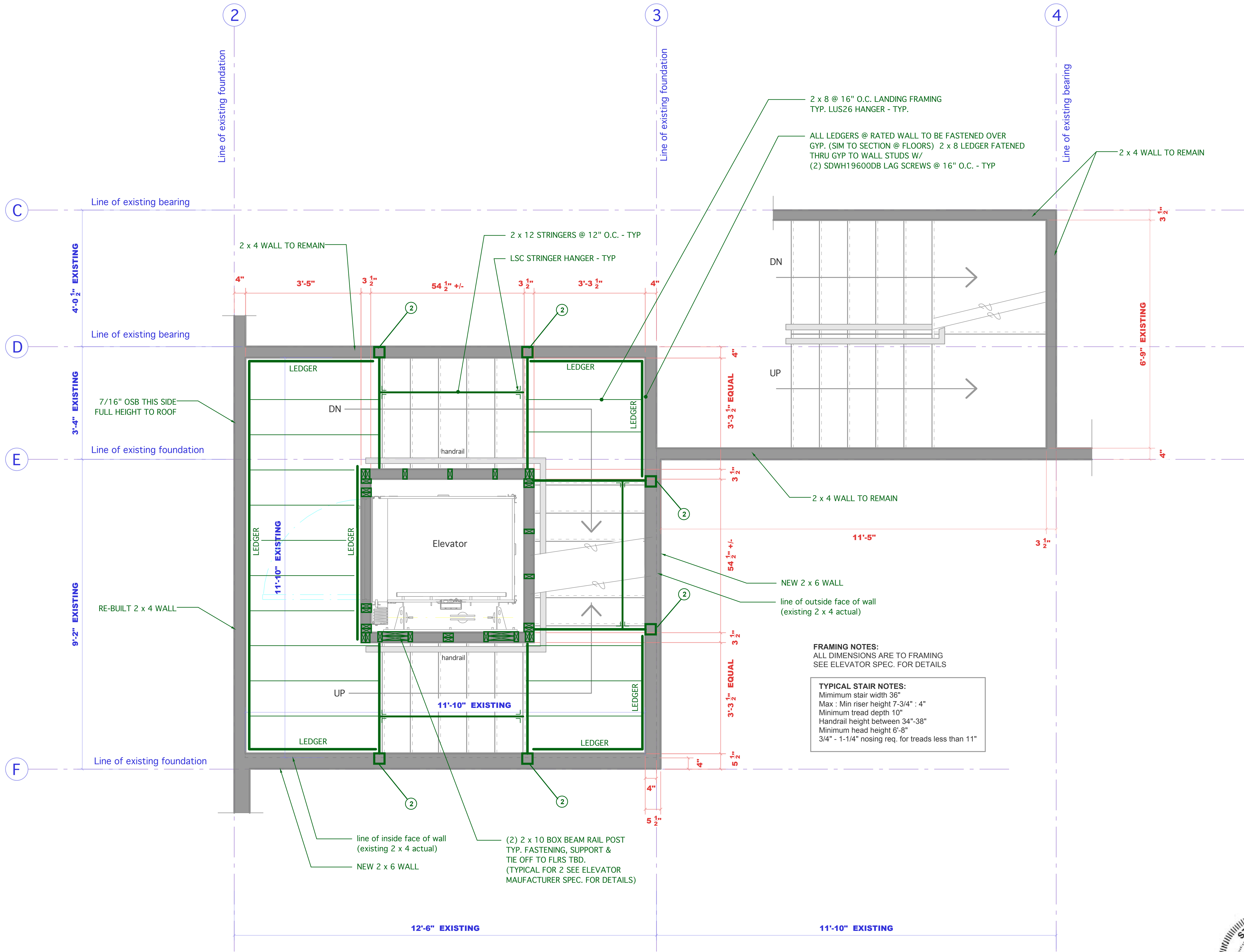
1 - TYPICAL ELEVATOR & STAIR PLAN DETAIL 3/4" = 1'-0"
