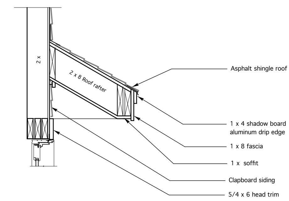
5 SECTION DETAIL scale: 3/4" = 1'-0"
