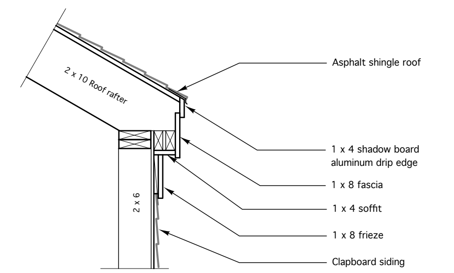
6 SECTION DETAIL scale: 3/4" = 1'-0"
