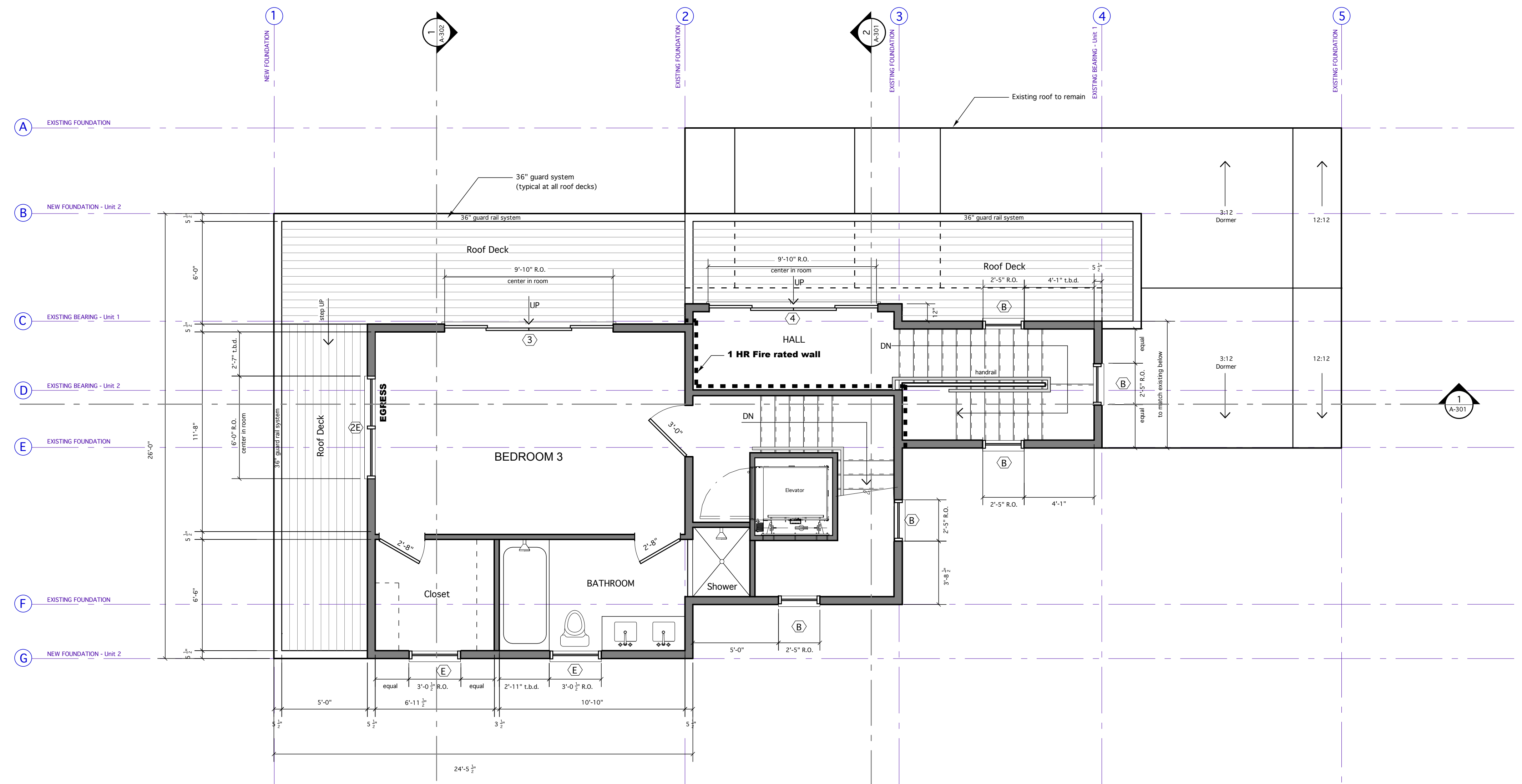
PROPOSED FOURTH FLOOR PLAN
