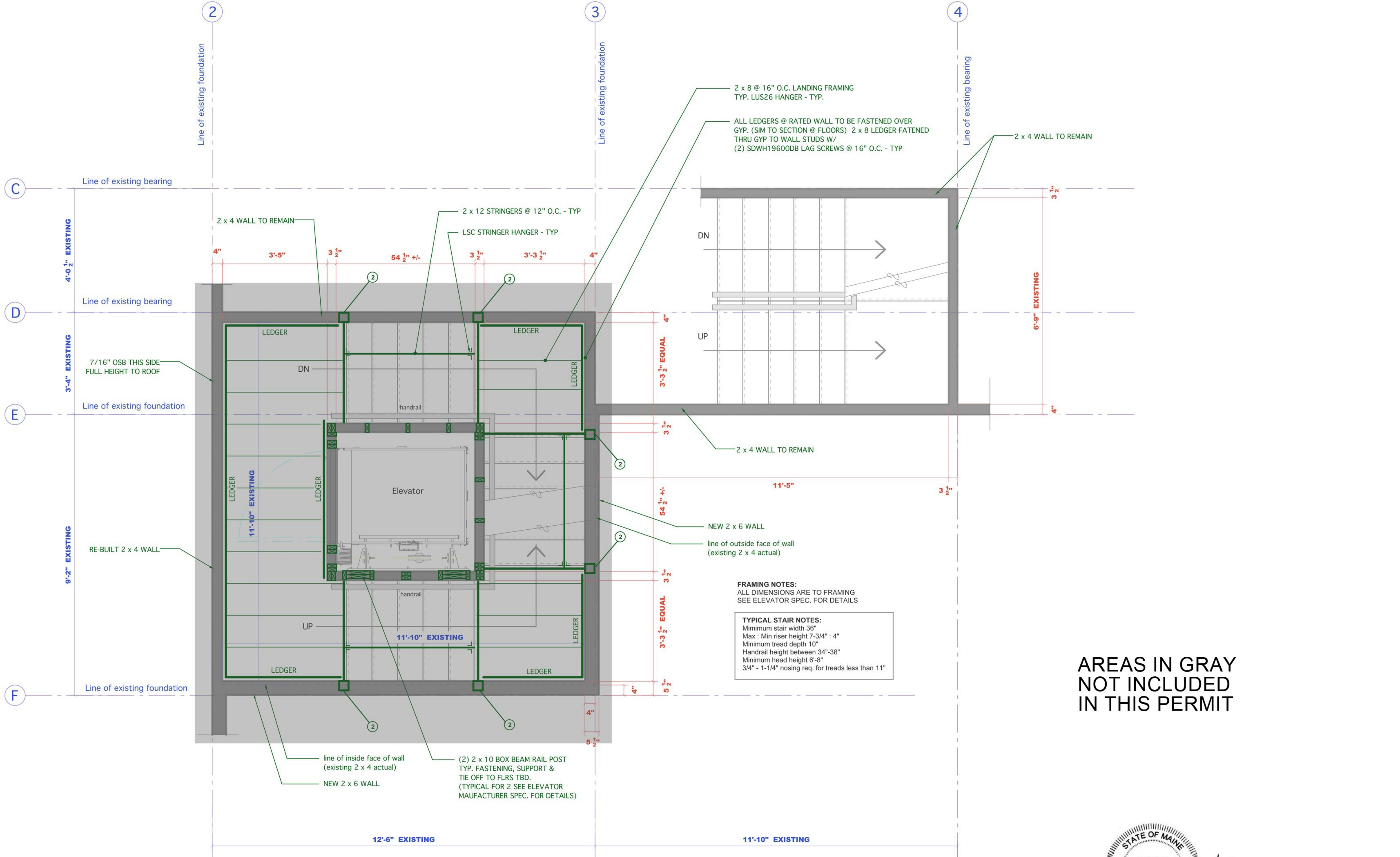
1 - TYPICAL ELEVATOR & STAIR PLAN DETAIL 3/4" = 1'-0"
