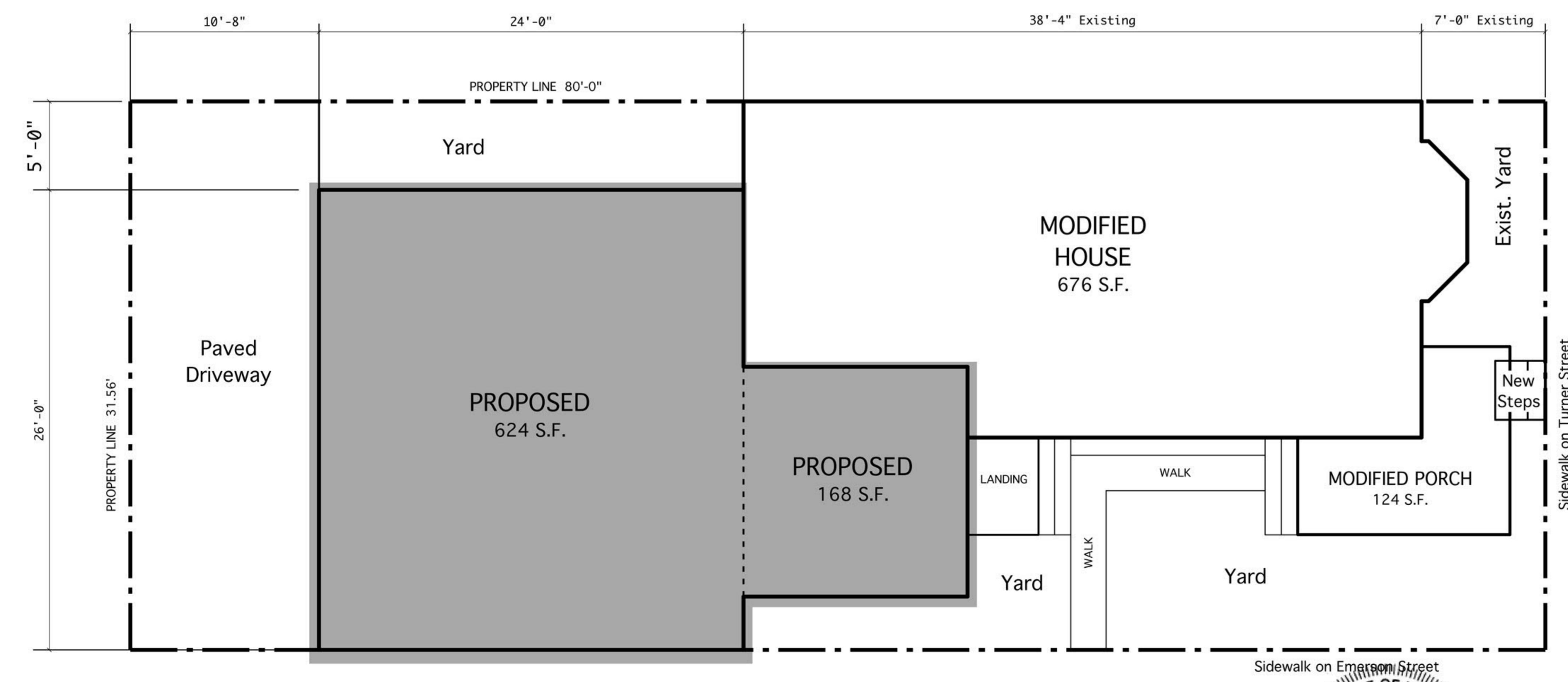
PROPOSED PLOT PLAN
