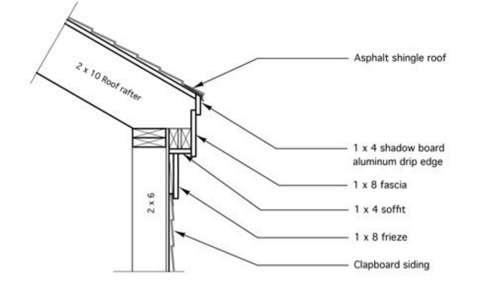
6 SECTION DETAIL scale: 3/4" = 1'-0"
