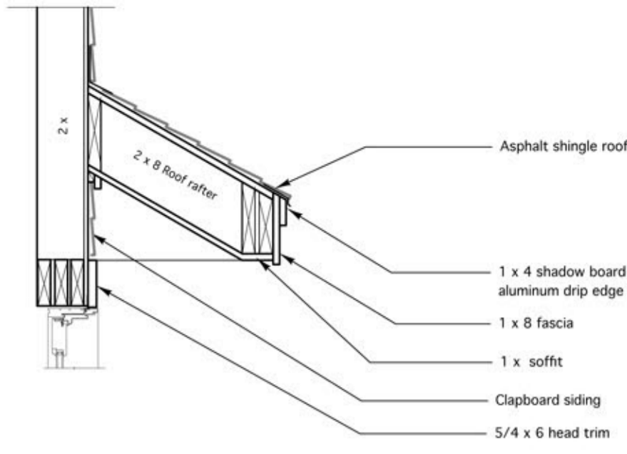
5 SECTION DETAIL scale: 3/4" = 1'-0"
