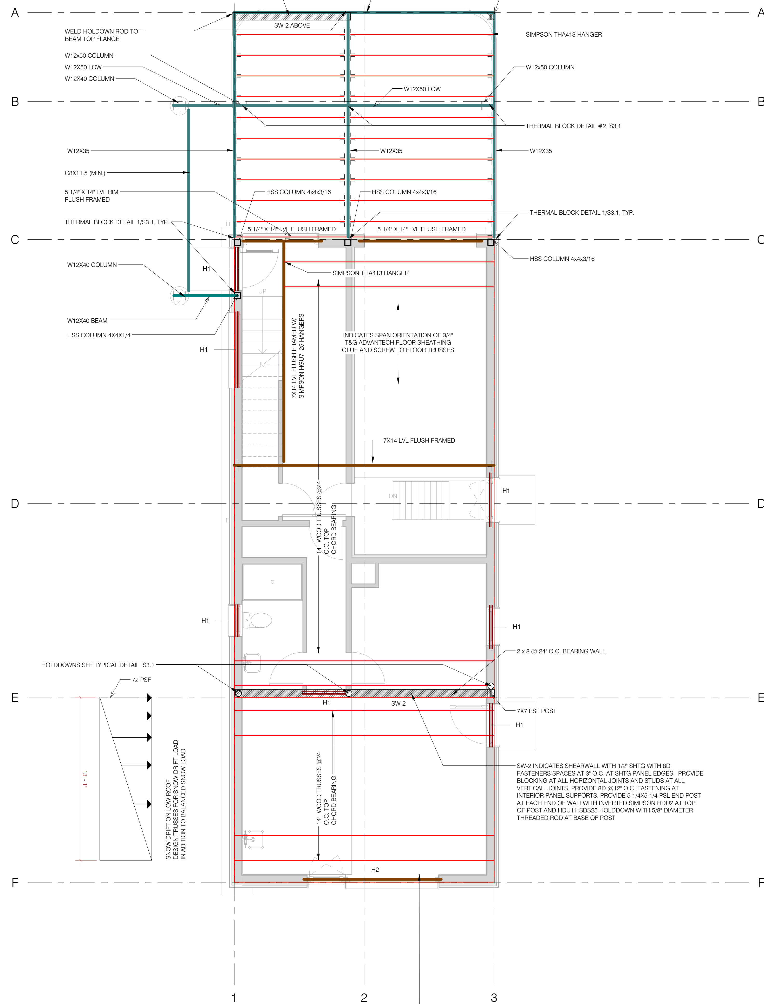
1 Second Floor Framing Over First Floor 1/4" = 1'-0"
