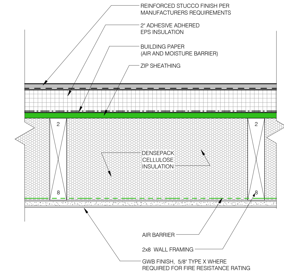
2 W3 - Exterior Wall With 2" EPS and Stucco Finish 3' = 1'-0"
