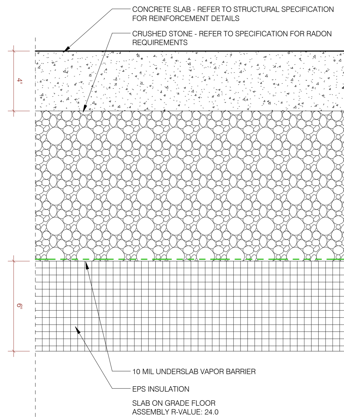
7 Assembly - First Floor Slab 3' = 1'-0"
