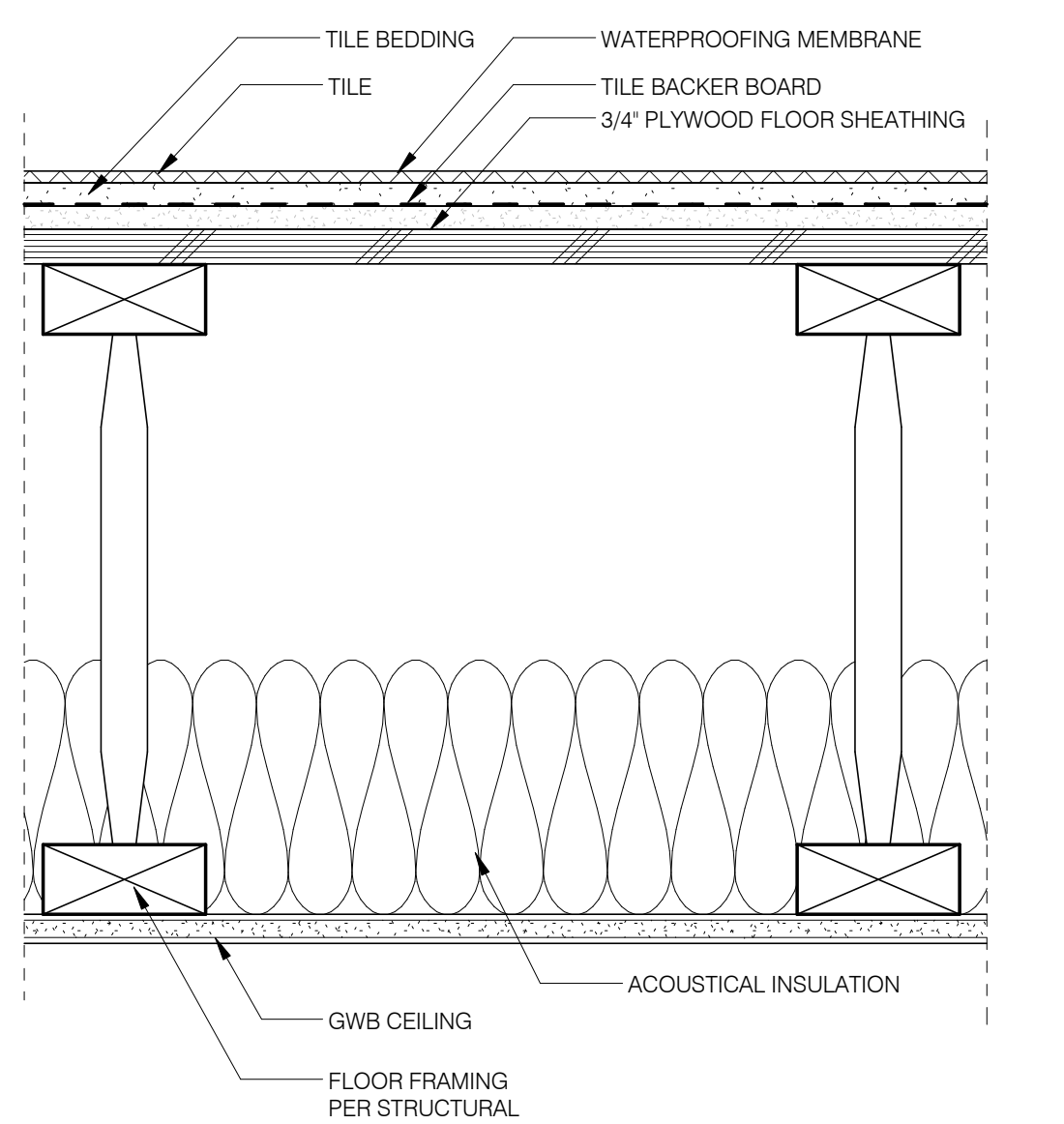
8 Assembly - Typical Second Floor 3' = 1'-0"
