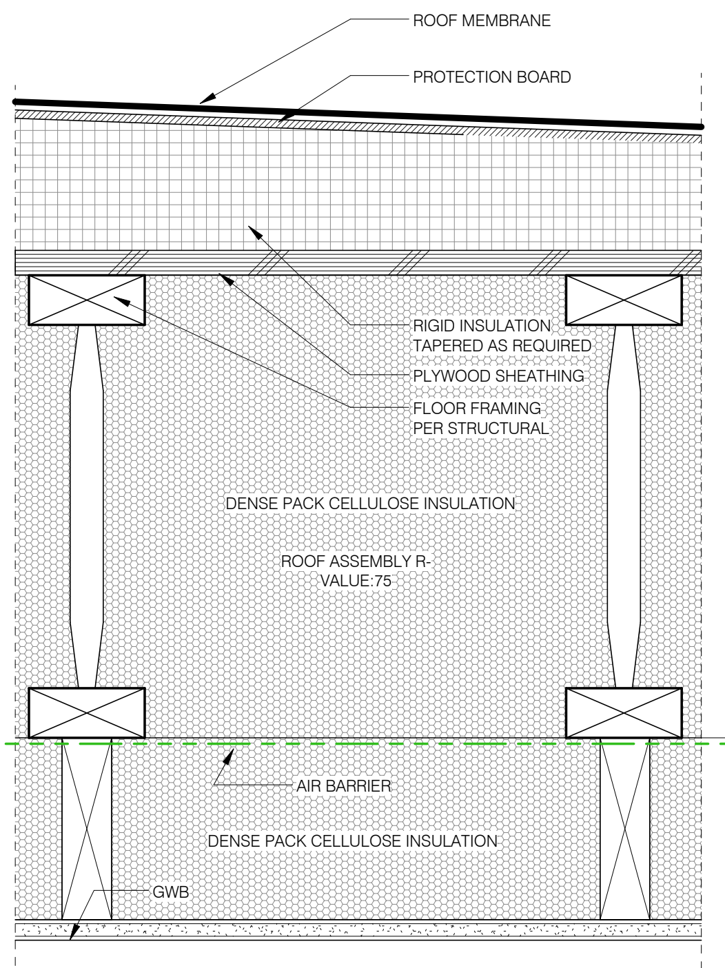
10 Assembly - Exterior Roof Deck 3' = 1'-0"
