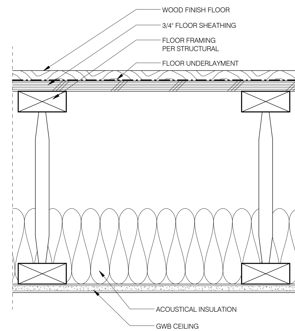
8 Assembly - Typical Second Floor 3' = 1'-0"
