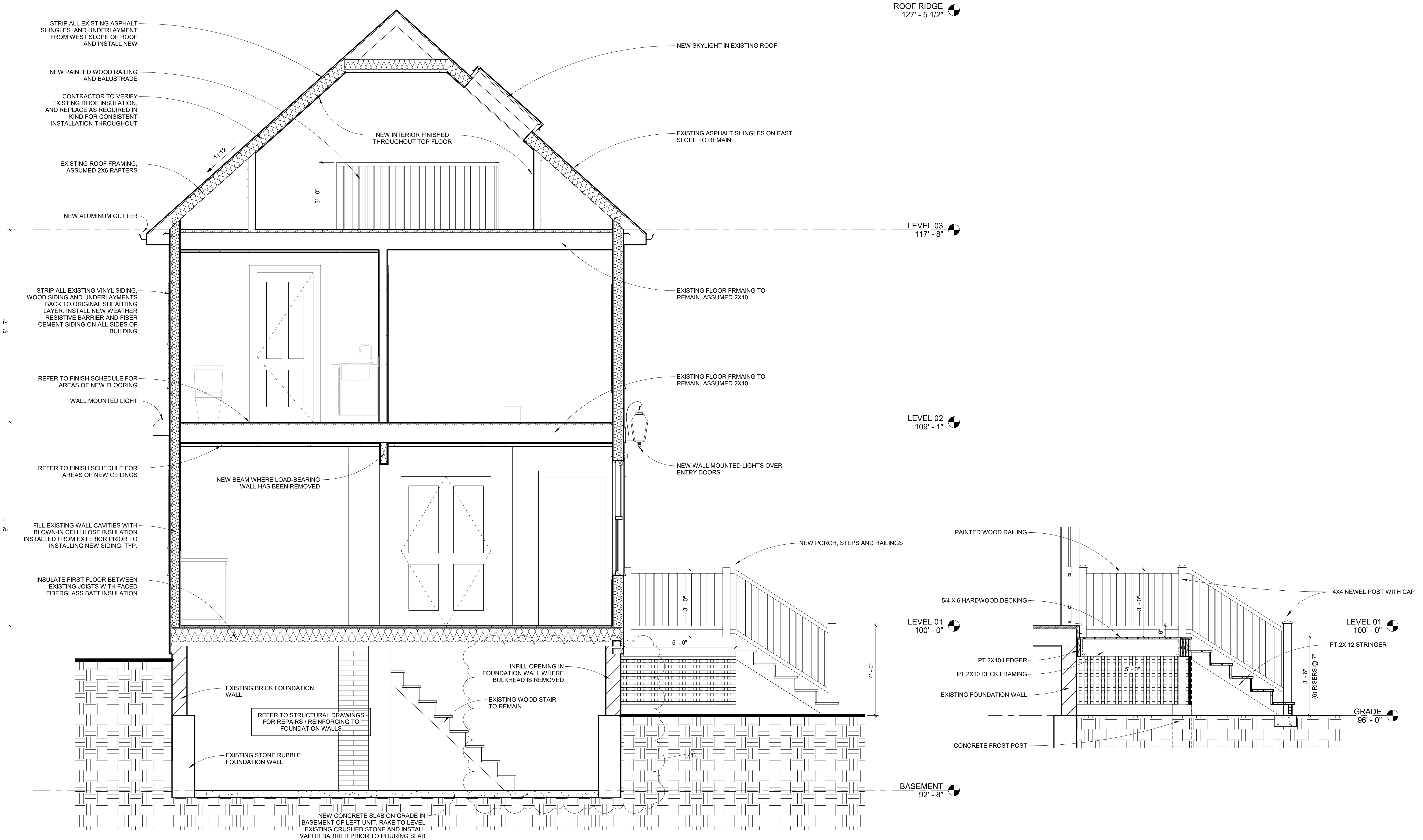
① Cross Section 1/2" = 1'-0"
