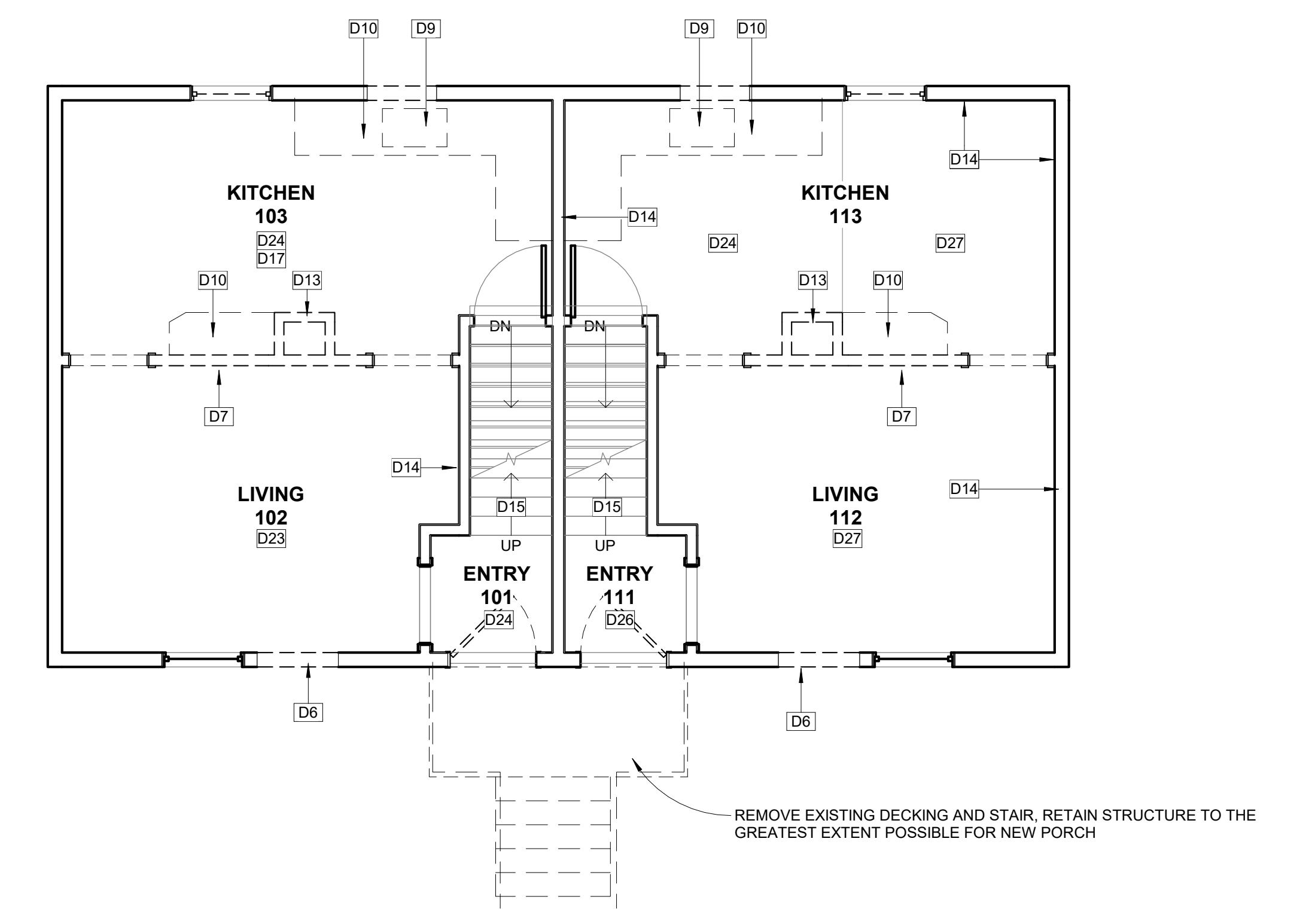
③ Level 01 Demo Floor Plan 1/4" = 1'-0"
