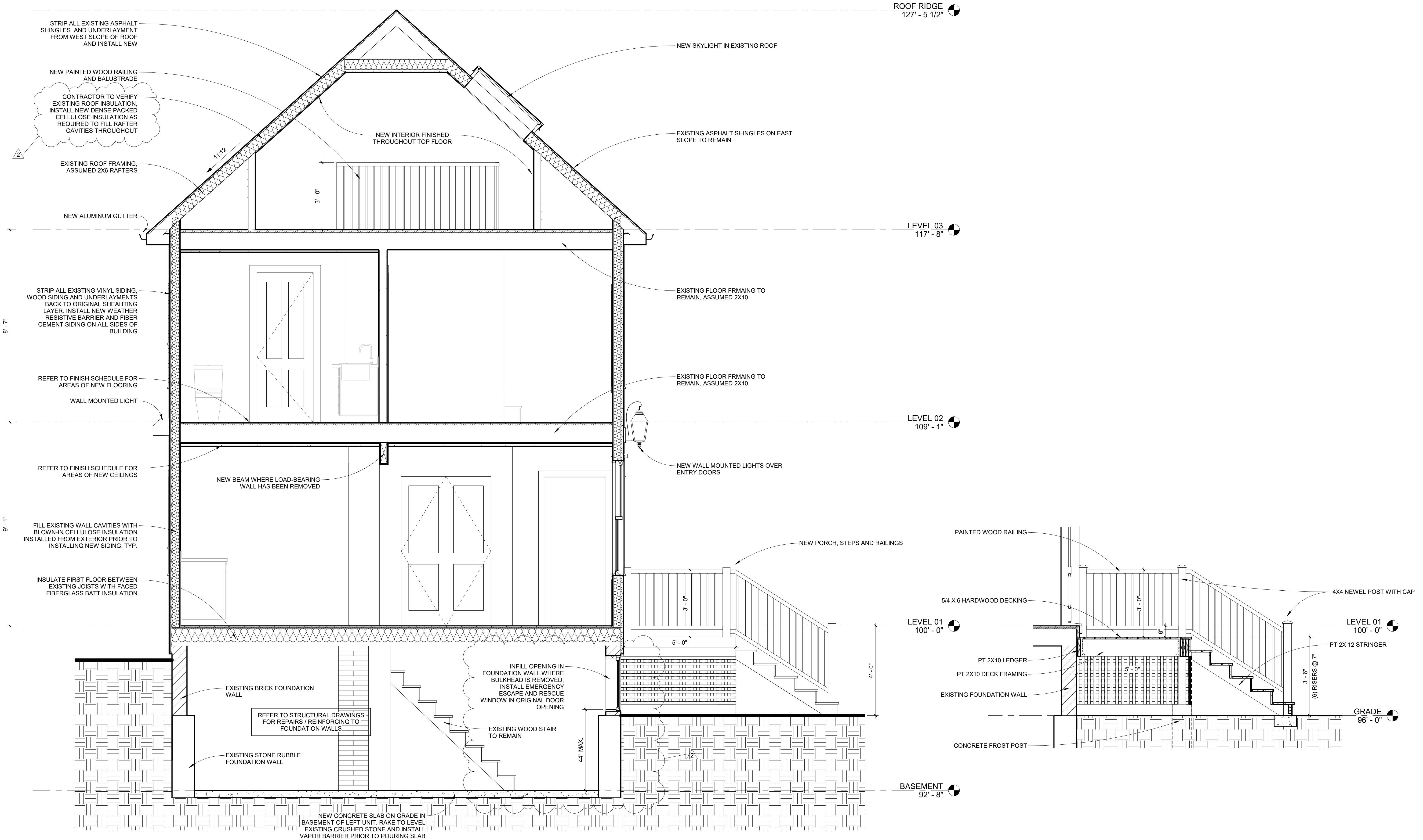
1 Cross Section 1/2" = 1'-0"
