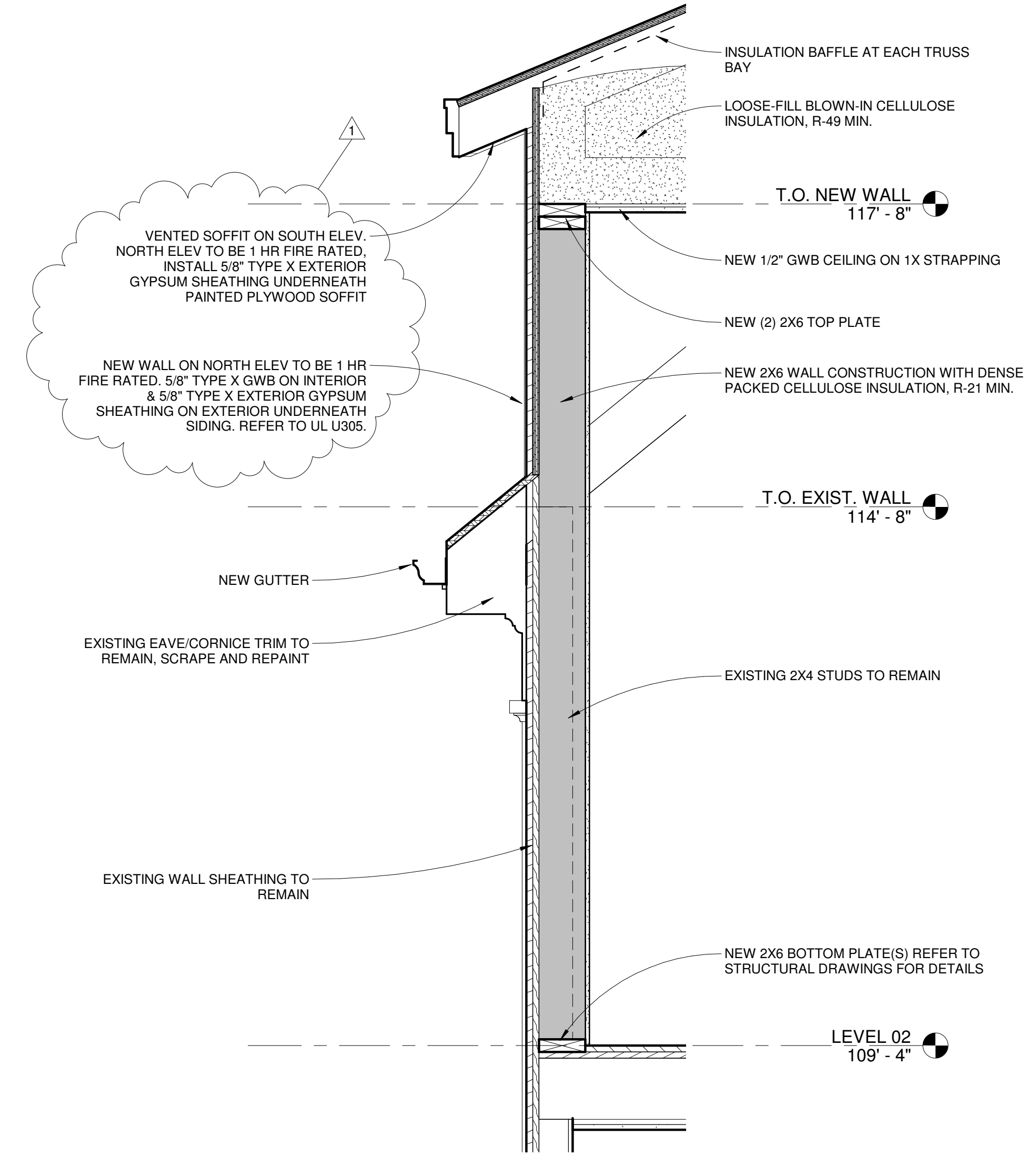
3 NEW DORMER WALL DETAIL SECTION 1" = 1'-0"
