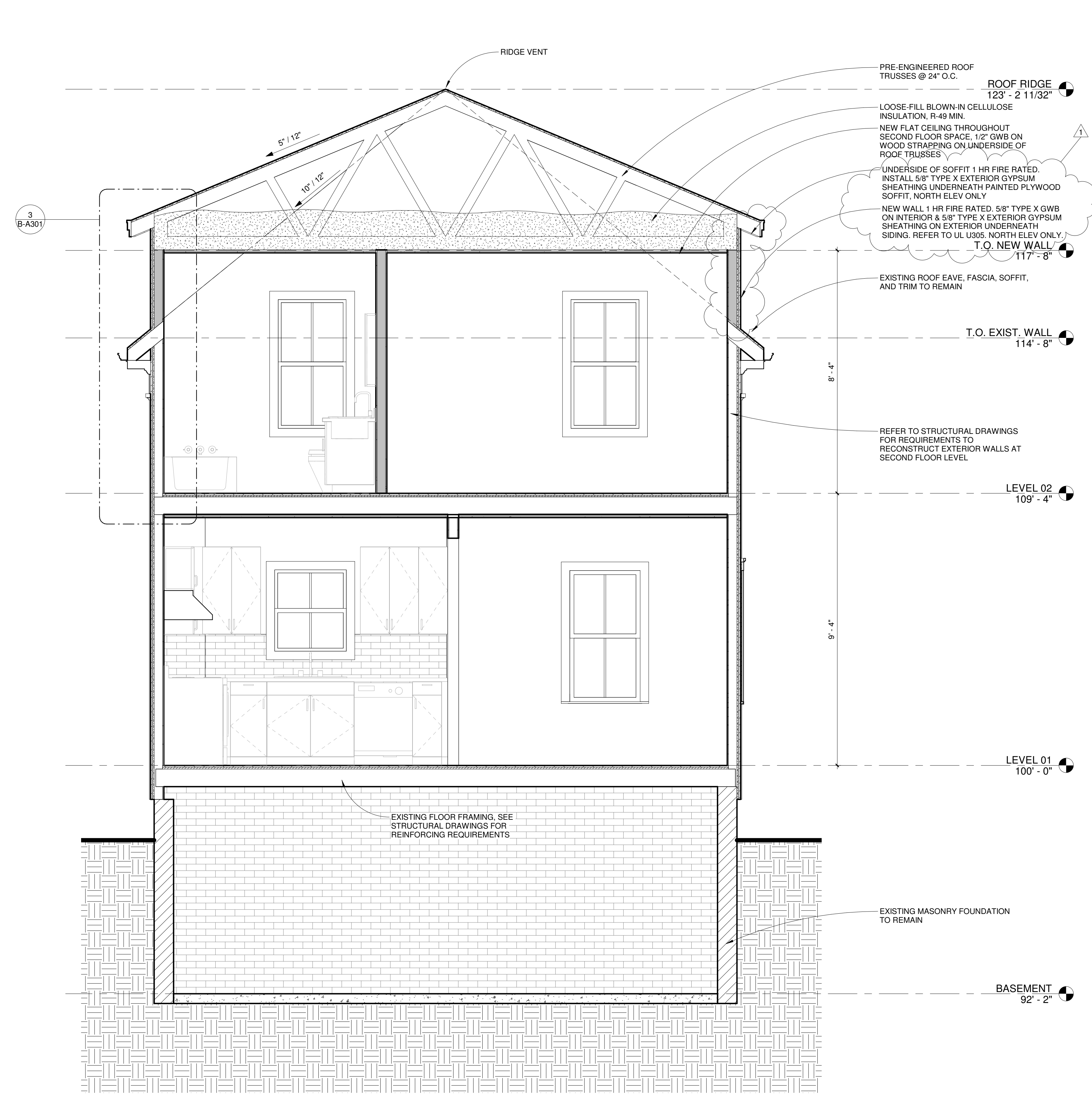
1 Cross Section 1/2" = 1'-0"
