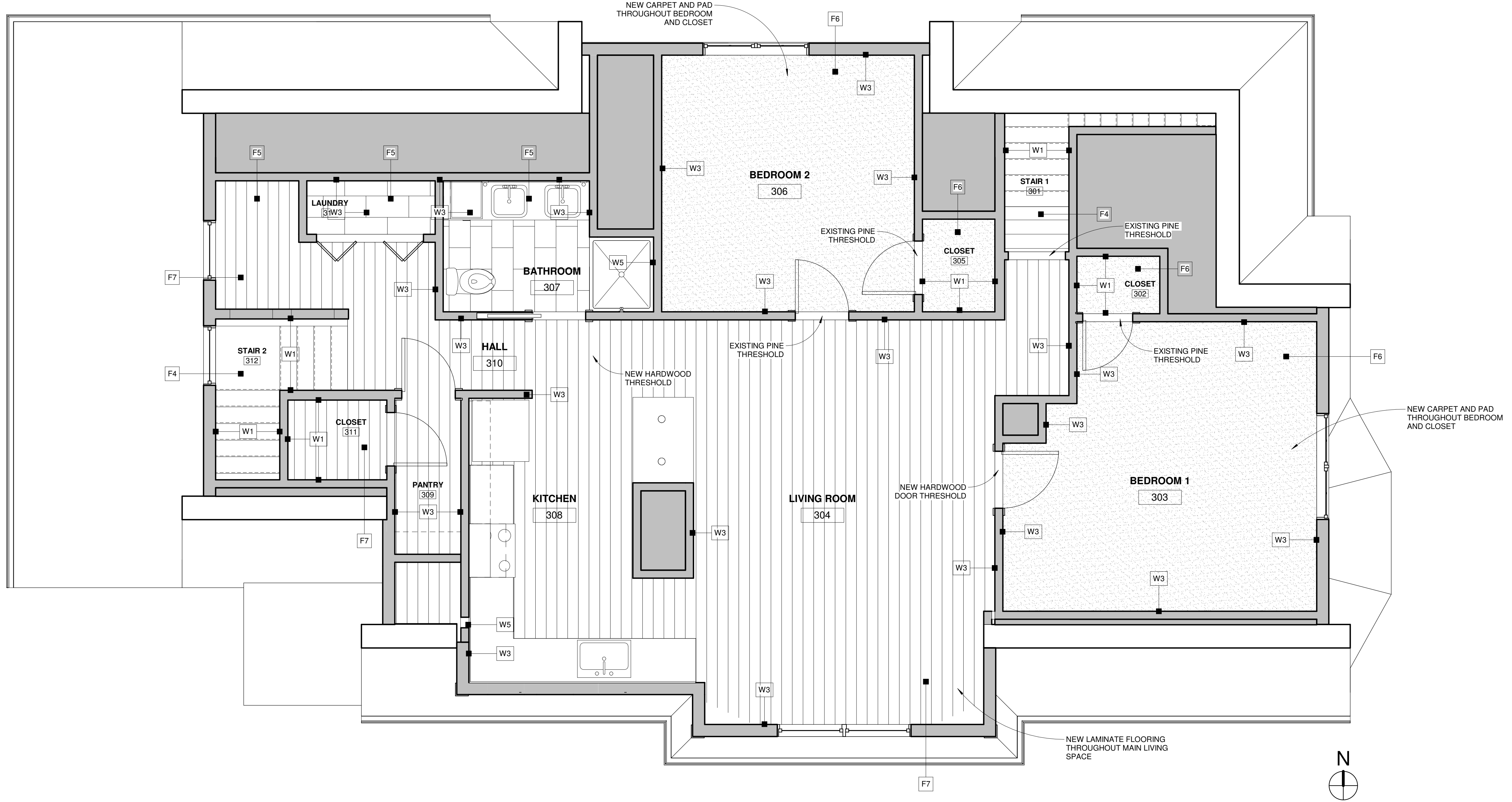
1 UNIT 3 - FINISH PLAN 3/8" = 1'-0"
